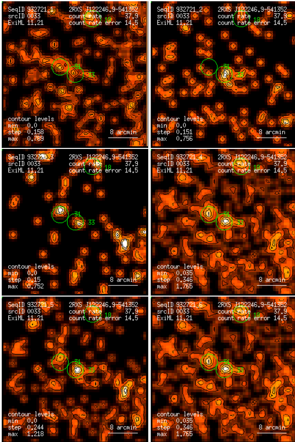
Figure 33: RASS 932721: detection 0033: band rate images, Gaussian filter: (1) PSPC channels 11 – 41, (2) 52 – 90, (3) 91 – 201, (4) 11 – 235, (5) 52 – 201, (6) 11 – 201. Broad band rates in counts/ks. Band rate contour levels in counts/ks/arcmin 2 .
