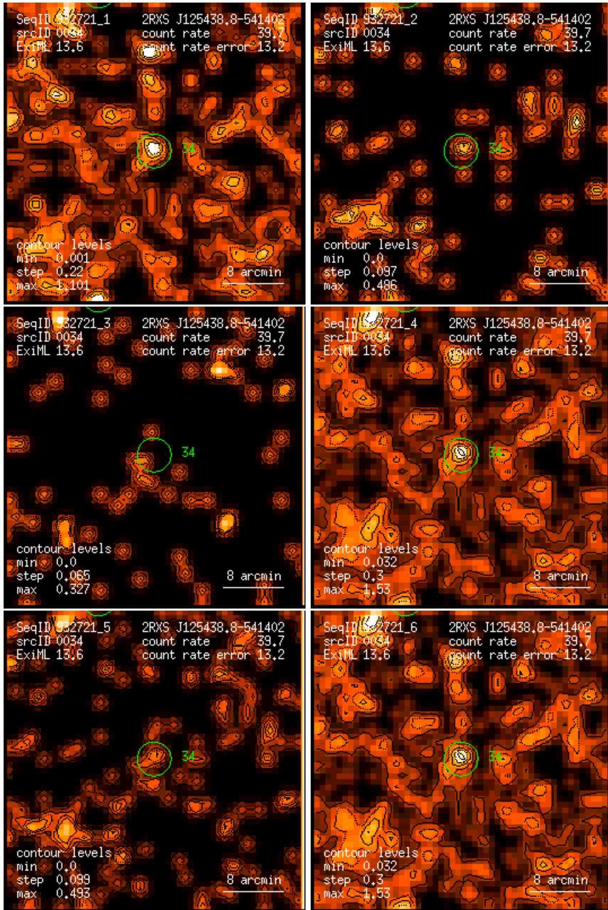
Figure 34: RASS 932721: detection 0034: band rate images, Gaussian filter: (1) PSPC channels 11 – 41, (2) 52 – 90, (3) 91 – 201, (4) 11 – 235, (5) 52 – 201, (6) 11 – 201. Broad band rates in counts/ks. Band rate contour levels in counts/ks/arcmin 2 .
