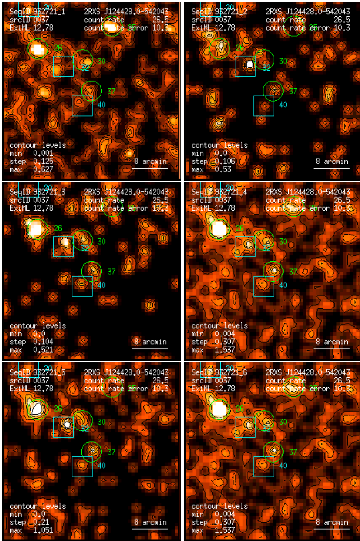
Figure 37: RASS 932721: detection 0037: band rate images, Gaussian filter: (1) PSPC channels 11 – 41, (2) 52 – 90, (3) 91 – 201, (4) 11 – 235, (5) 52 – 201, (6) 11 – 201. Broad band rates in counts/ks. Band rate contour levels in counts/ks/arcmin 2 .
