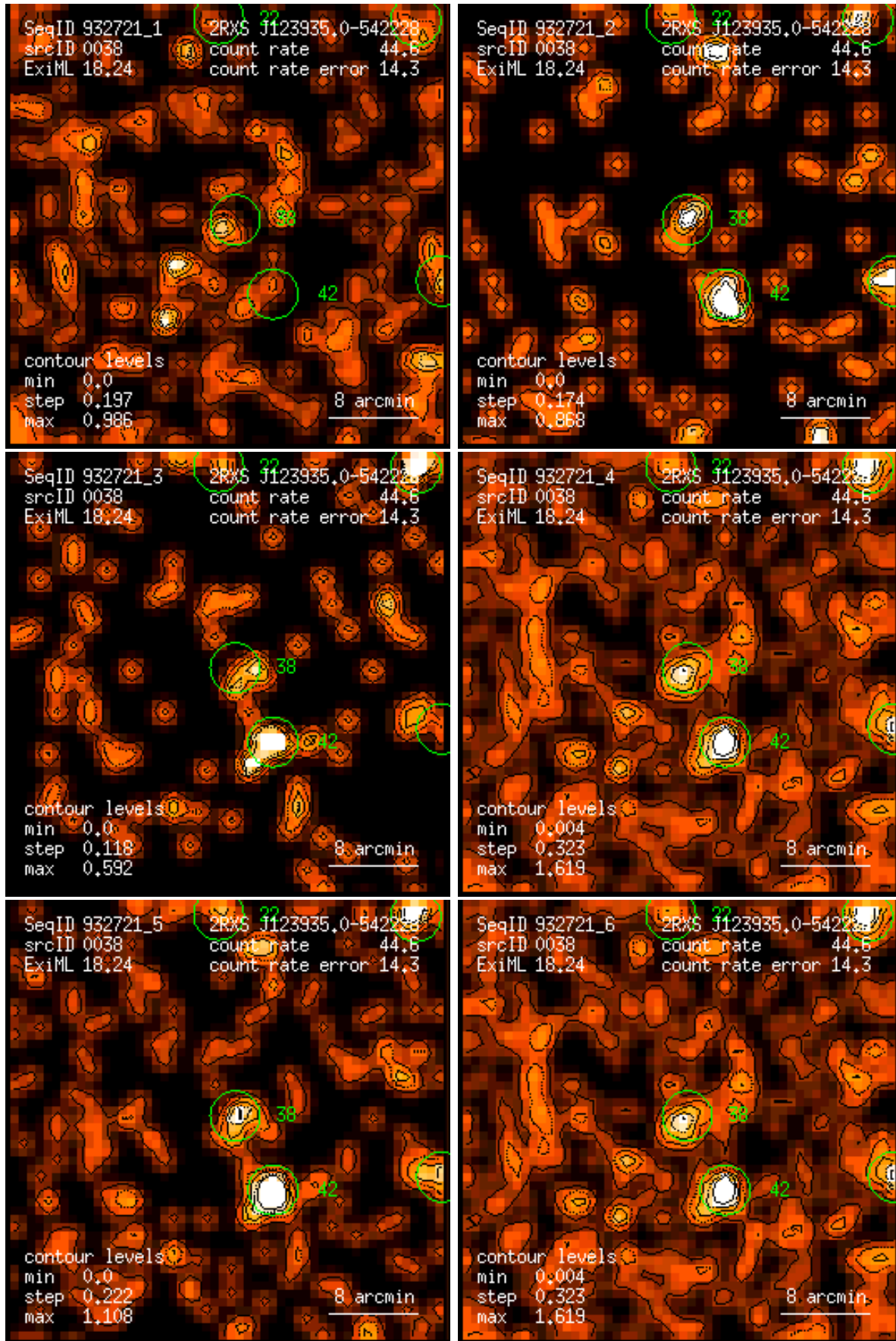
Figure 38: RASS 932721: detection 0038: band rate images, Gaussian filter: (1) PSPC channels 11 – 41, (2) 52 – 90, (3) 91 – 201, (4) 11 – 235, (5) 52 – 201, (6) 11 – 201. Broad band rates in counts/ks. Band rate contour levels in counts/ks/arcmin 2 .
