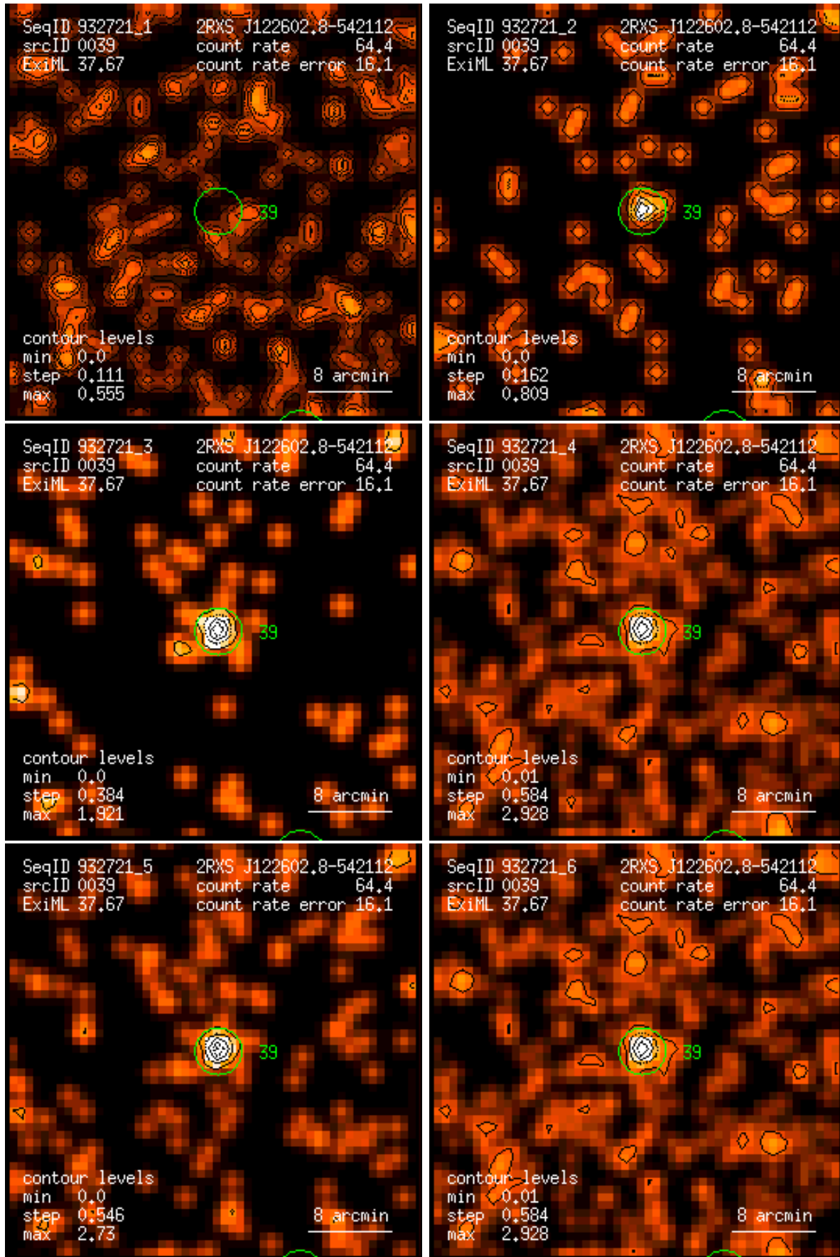
Figure 39: RASS 932721: detection 0039: band rate images, Gaussian filter: (1) PSPC channels 11 – 41, (2) 52 – 90, (3) 91 – 201, (4) 11 – 235, (5) 52 – 201, (6) 11 – 201. Broad band rates in counts/ks. Band rate contour levels in counts/ks/arcmin 2 .
