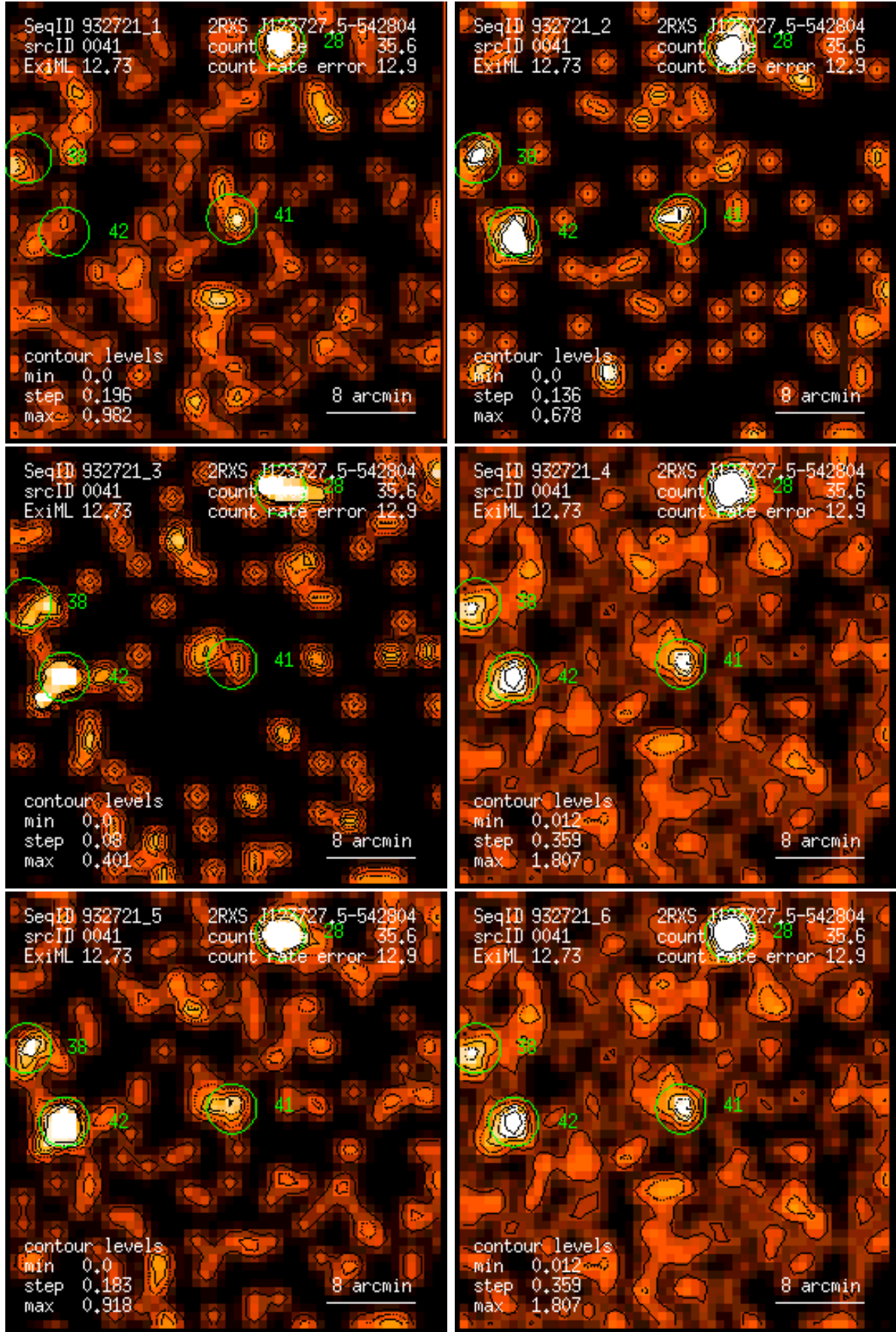
Figure 41: RASS 932721: detection 0041: band rate images, Gaussian filter: (1) PSPC channels 11 – 41, (2) 52 – 90, (3) 91 – 201, (4) 11 – 235, (5) 52 – 201, (6) 11 – 201. Broad band rates in counts/ks. Band rate contour levels in counts/ks/arcmin 2 .
