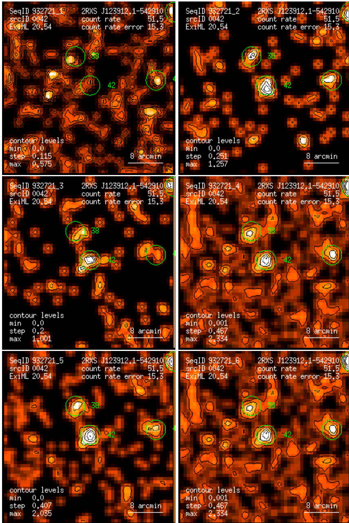
Figure 42: RASS 932721: detection 0042: band rate images, Gaussian filter: (1) PSPC channels 11 – 41, (2) 52 – 90, (3) 91 – 201, (4) 11 – 235, (5) 52 – 201, (6) 11 – 201. Broad band rates in counts/ks. Band rate contour levels in counts/ks/arcmin 2 .
