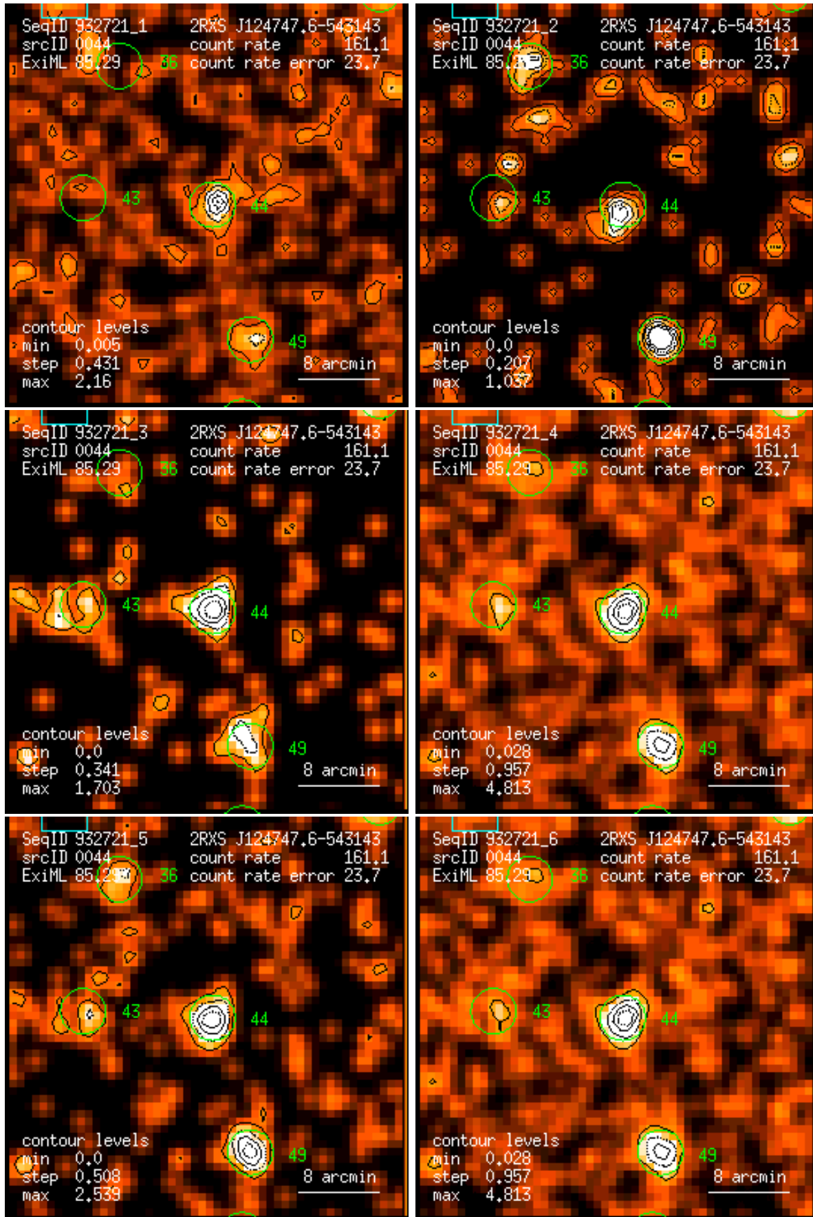
Figure 44: RASS 932721: detection 0044: band rate images, Gaussian filter: (1) PSPC channels 11 – 41, (2) 52 – 90, (3) 91 – 201, (4) 11 – 235, (5) 52 – 201, (6) 11 – 201. Broad band rates in counts/ks. Band rate contour levels in counts/ks/arcmin 2 .
