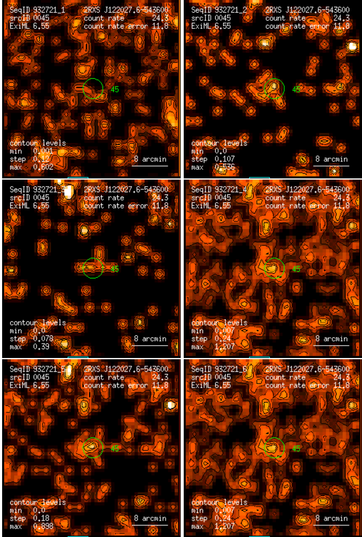
Figure 45: RASS 932721: detection 0045: band rate images, Gaussian filter: (1) PSPC channels 11 – 41, (2) 52 – 90, (3) 91 – 201, (4) 11 – 235, (5) 52 – 201, (6) 11 – 201. Broad band rates in counts/ks. Band rate contour levels in counts/ks/arcmin 2 .
