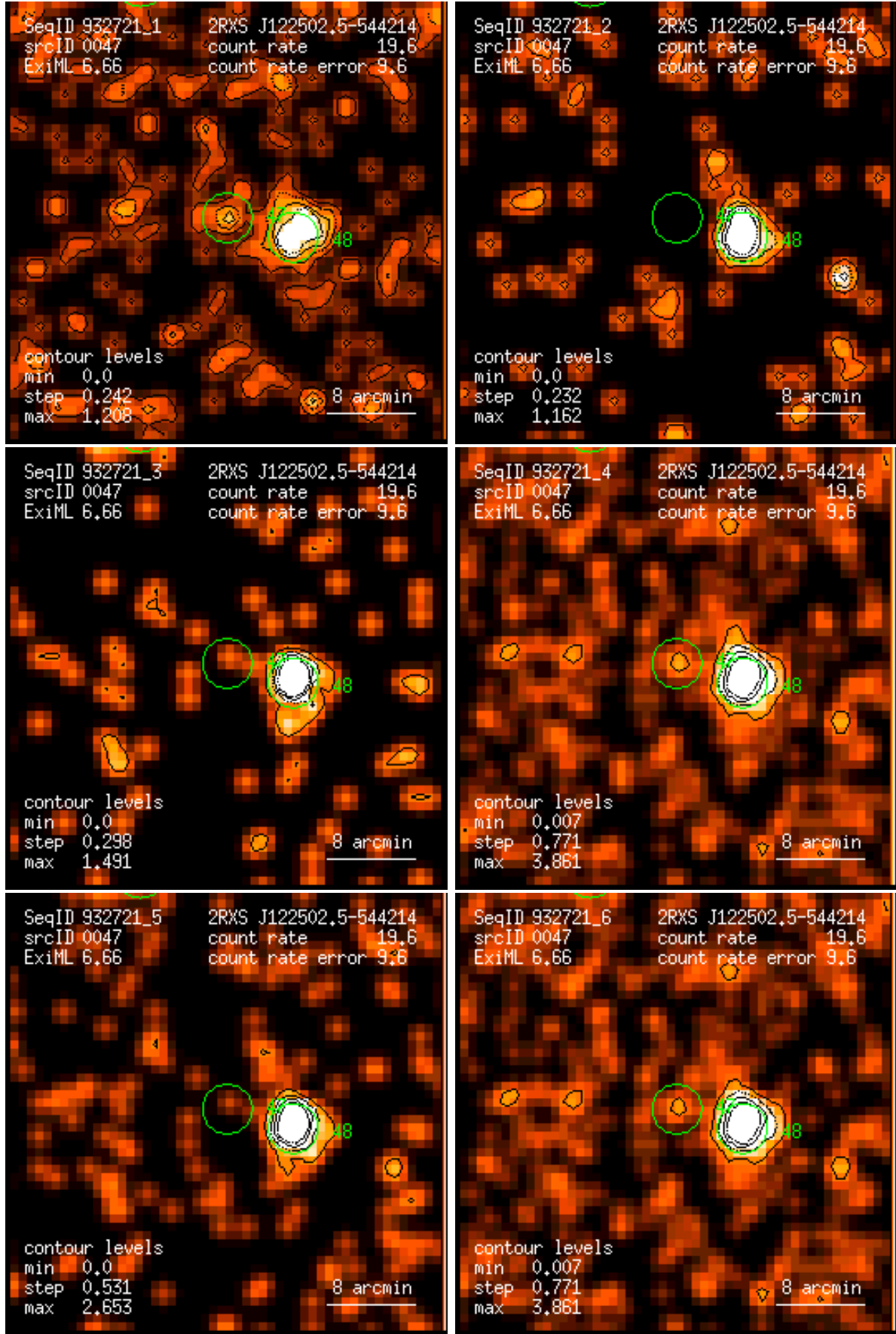
Figure 47: RASS 932721: detection 0047: band rate images, Gaussian filter: (1) PSPC channels 11 – 41, (2) 52 – 90, (3) 91 – 201, (4) 11 – 235, (5) 52 – 201, (6) 11 – 201. Broad band rates in counts/ks. Band rate contour levels in counts/ks/arcmin 2 .
