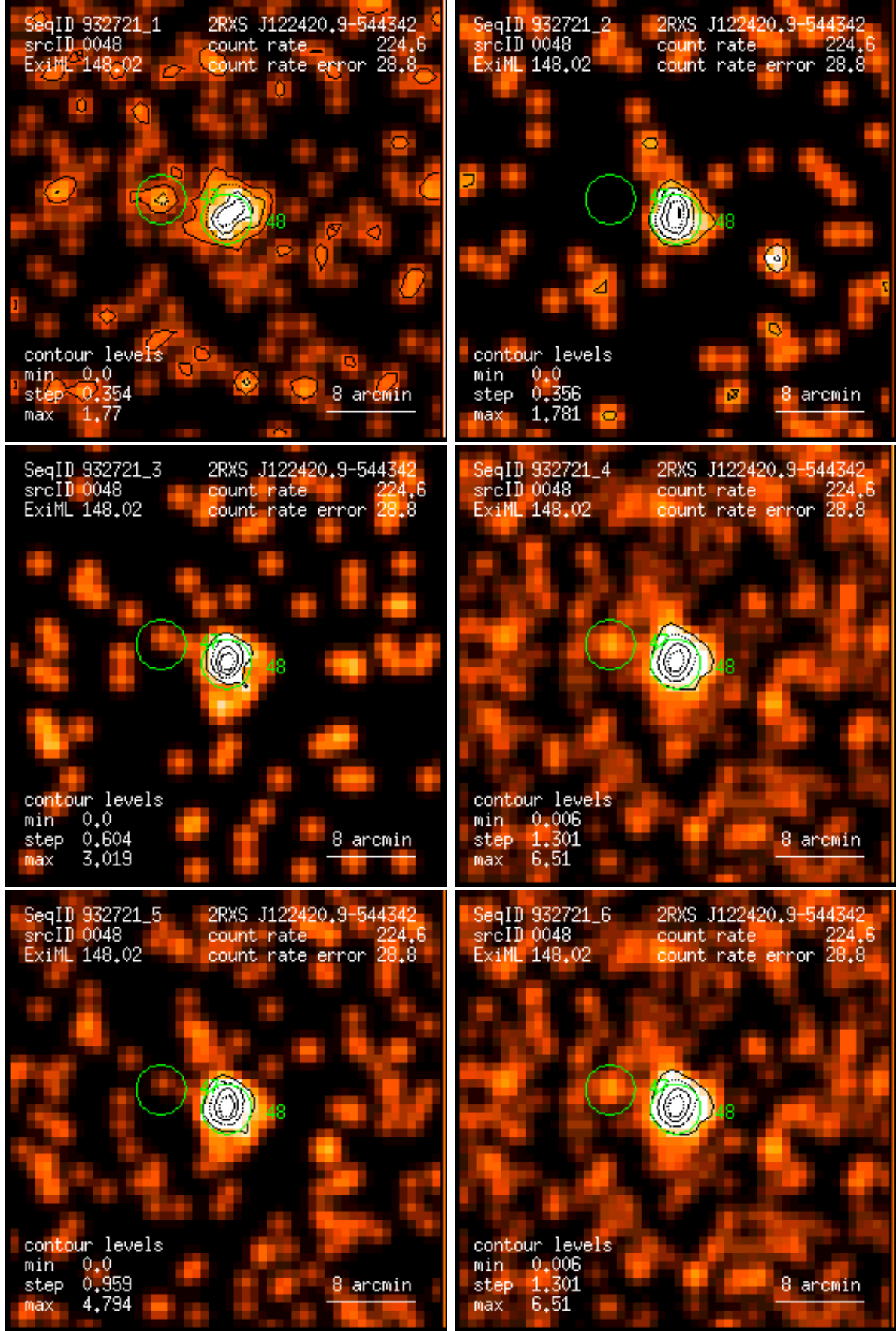
Figure 48: RASS 932721: detection 0048: band rate images, Gaussian filter: (1) PSPC channels 11 – 41, (2) 52 – 90, (3) 91 – 201, (4) 11 – 235, (5) 52 – 201, (6) 11 – 201. Broad band rates in counts/ks. Band rate contour levels in counts/ks/arcmin 2 .
