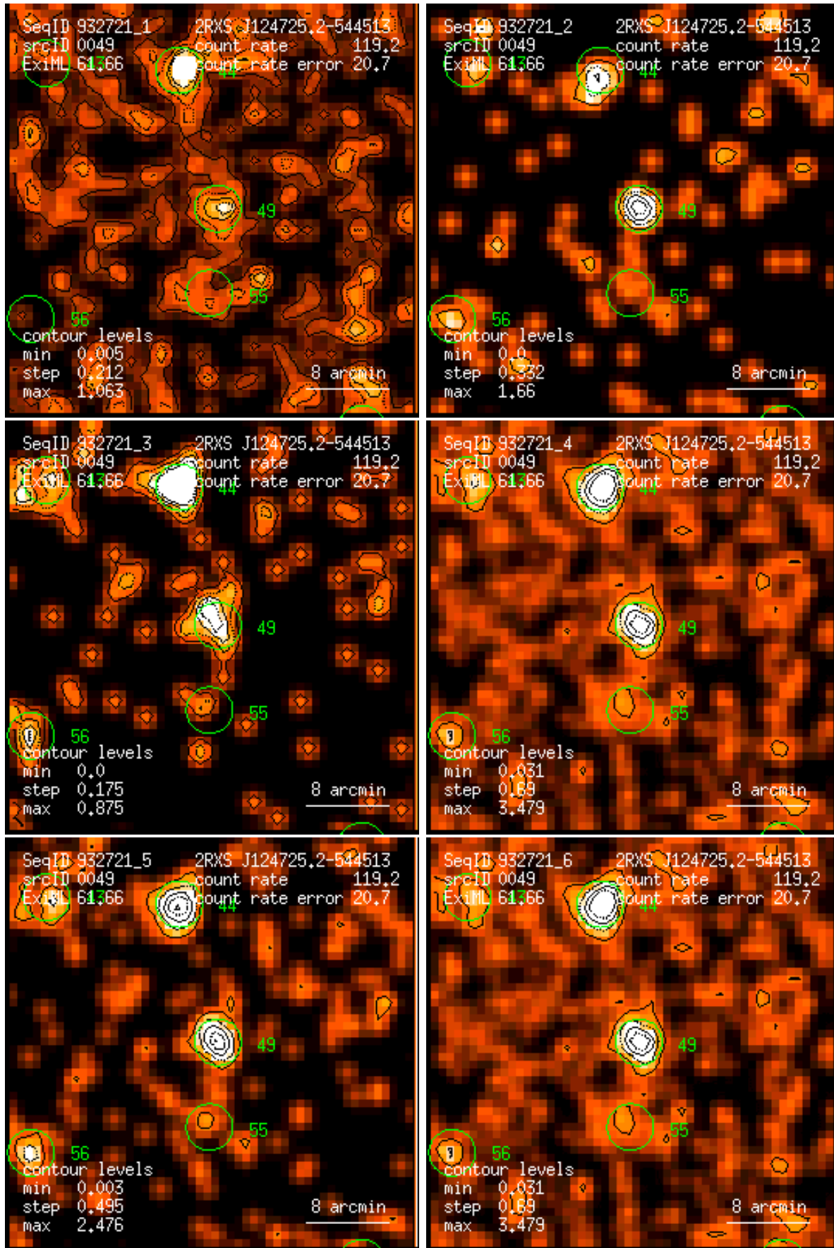
Figure 49: RASS 932721: detection 0049: band rate images, Gaussian filter: (1) PSPC channels 11 – 41, (2) 52 – 90, (3) 91 – 201, (4) 11 – 235, (5) 52 – 201, (6) 11 – 201. Broad band rates in counts/ks. Band rate contour levels in counts/ks/arcmin 2 .
