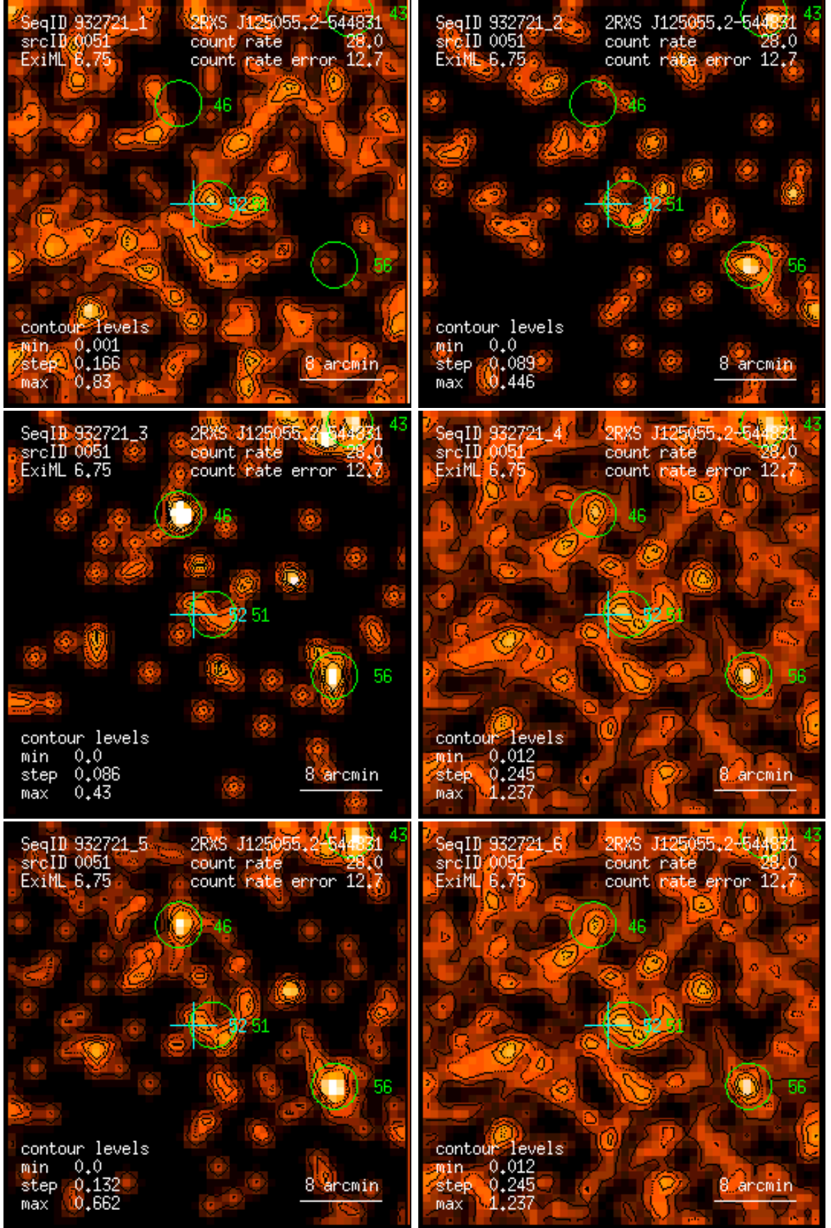
Figure 51: RASS 932721: detection 0051: band rate images, Gaussian filter: (1) PSPC channels 11 – 41, (2) 52 – 90, (3) 91 – 201, (4) 11 – 235, (5) 52 – 201, (6) 11 – 201. Broad band rates in counts/ks. Band rate contour levels in counts/ks/arcmin 2 .
