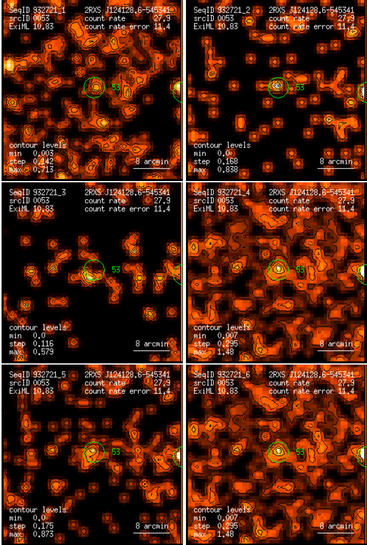
Figure 53: RASS 932721: detection 0053: band rate images, Gaussian filter: (1) PSPC channels 11 – 41, (2) 52 – 90, (3) 91 – 201, (4) 11 – 235, (5) 52 – 201, (6) 11 – 201. Broad band rates in counts/ks. Band rate contour levels in counts/ks/arcmin 2 .
