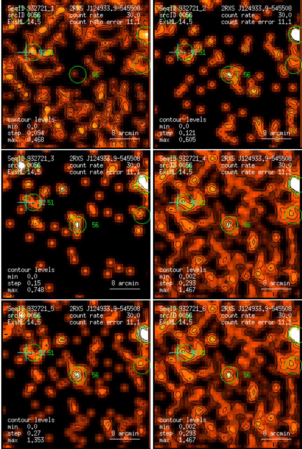
Figure 56: RASS 932721: detection 0056: band rate images, Gaussian filter: (1) PSPC channels 11 – 41, (2) 52 – 90, (3) 91 – 201, (4) 11 – 235, (5) 52 – 201, (6) 11 – 201. Broad band rates in counts/ks. Band rate contour levels in counts/ks/arcmin 2 .
