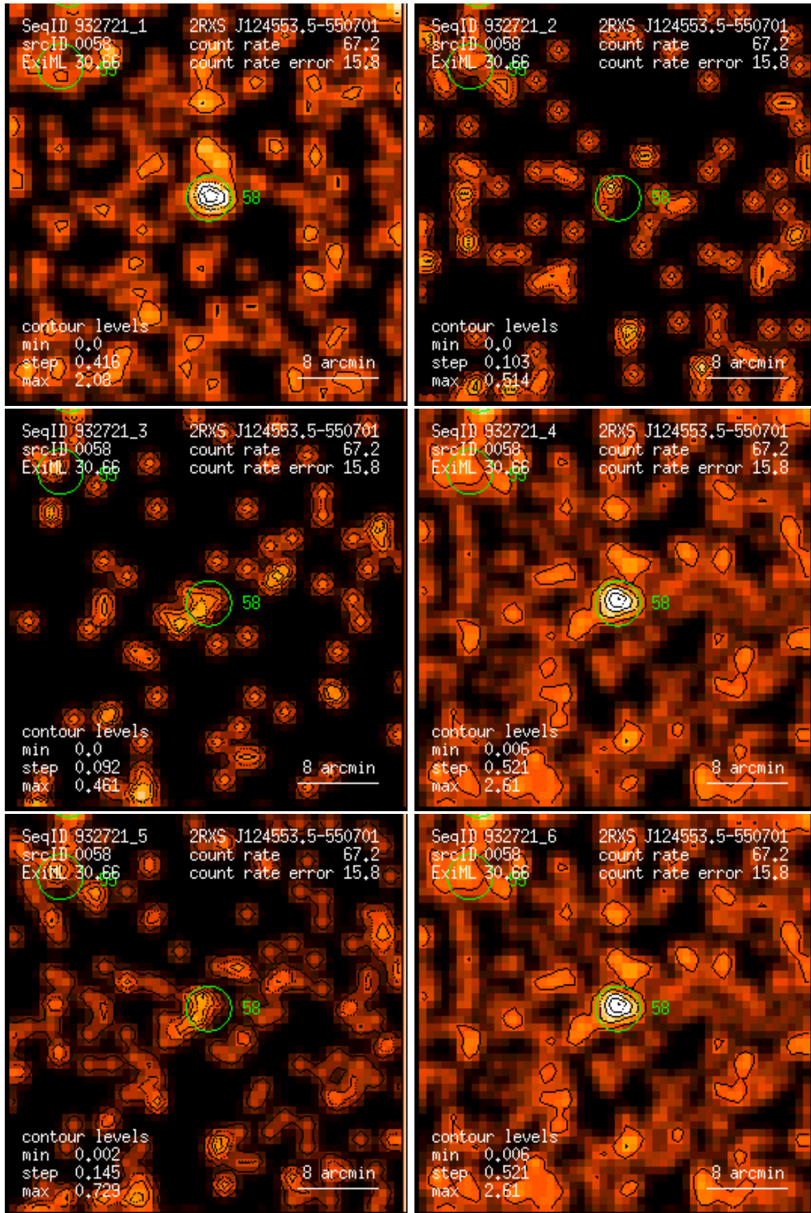
Figure 58: RASS 932721: detection 0058: band rate images, Gaussian filter: (1) PSPC channels 11 – 41, (2) 52 – 90, (3) 91 – 201, (4) 11 – 235, (5) 52 – 201, (6) 11 – 201. Broad band rates in counts/ks. Band rate contour levels in counts/ks/arcmin 2 .
