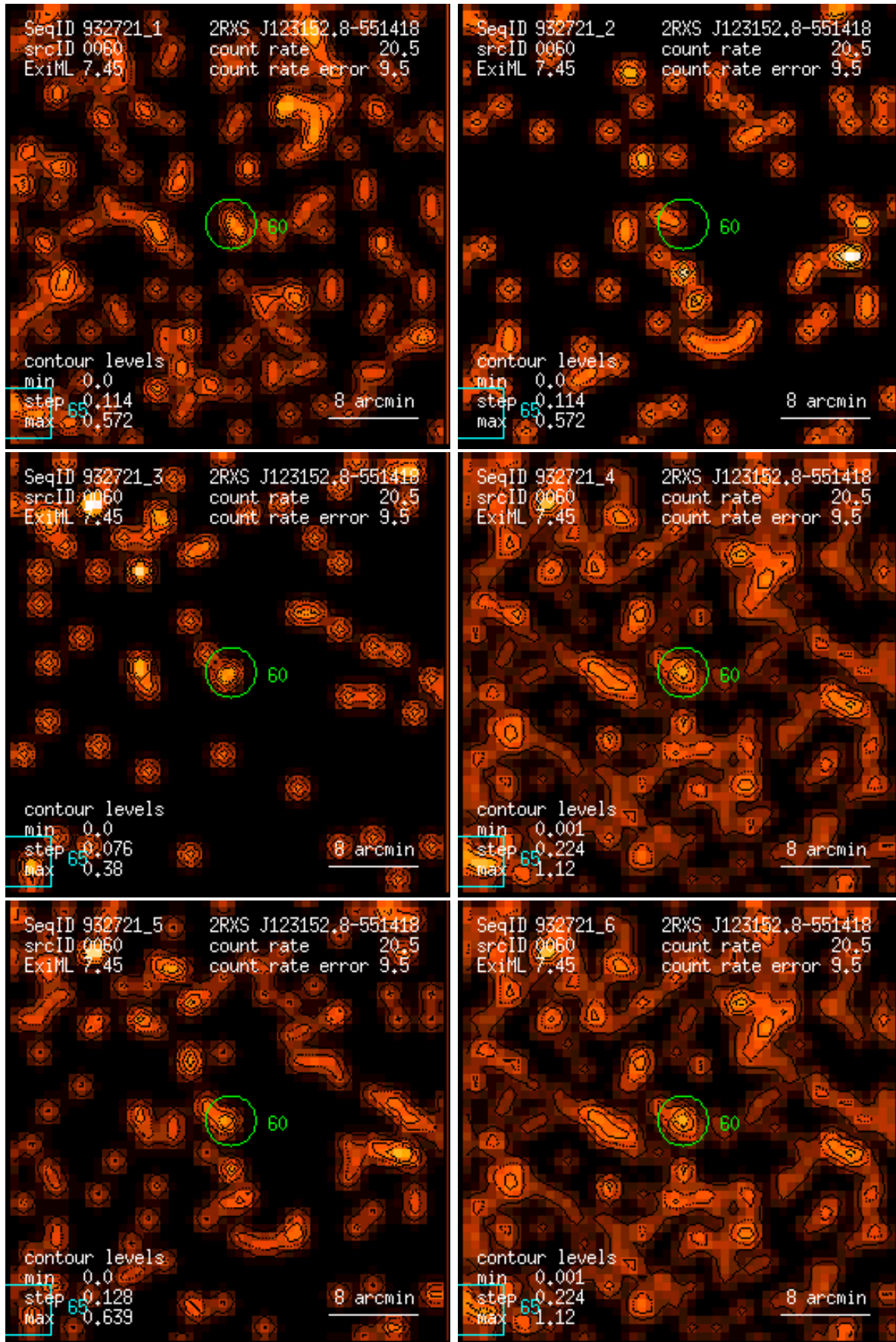
Figure 60: RASS 932721: detection 0060: band rate images, Gaussian filter: (1) PSPC channels 11 – 41, (2) 52 – 90, (3) 91 – 201, (4) 11 – 235, (5) 52 – 201, (6) 11 – 201. Broad band rates in counts/ks. Band rate contour levels in counts/ks/arcmin 2 .
