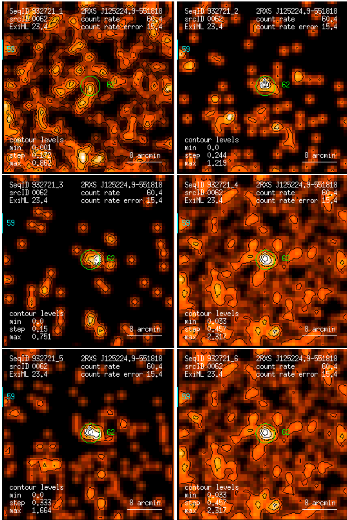
Figure 62: RASS 932721: detection 0062: band rate images, Gaussian filter: (1) PSPC channels 11 – 41, (2) 52 – 90, (3) 91 – 201, (4) 11 – 235, (5) 52 – 201, (6) 11 – 201. Broad band rates in counts/ks. Band rate contour levels in counts/ks/arcmin 2 .
