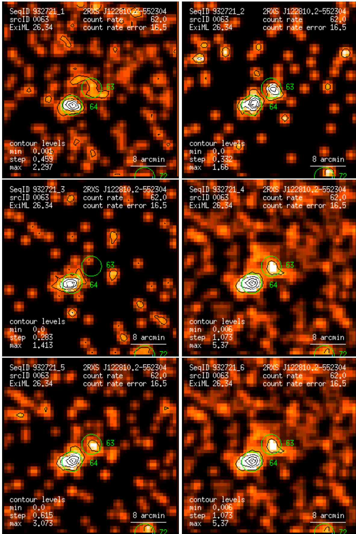
Figure 63: RASS 932721: detection 0063: band rate images, Gaussian filter: (1) PSPC channels 11 – 41, (2) 52 – 90, (3) 91 – 201, (4) 11 – 235, (5) 52 – 201, (6) 11 – 201. Broad band rates in counts/ks. Band rate contour levels in counts/ks/arcmin 2 .
