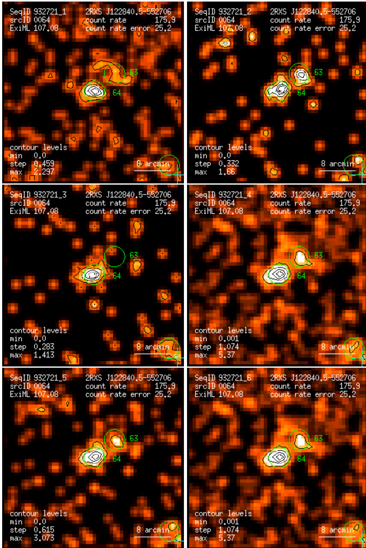
Figure 64: RASS 932721: detection 0064: band rate images, Gaussian filter: (1) PSPC channels 11 – 41, (2) 52 – 90, (3) 91 – 201, (4) 11 – 235, (5) 52 – 201, (6) 11 – 201. Broad band rates in counts/ks. Band rate contour levels in counts/ks/arcmin 2 .
