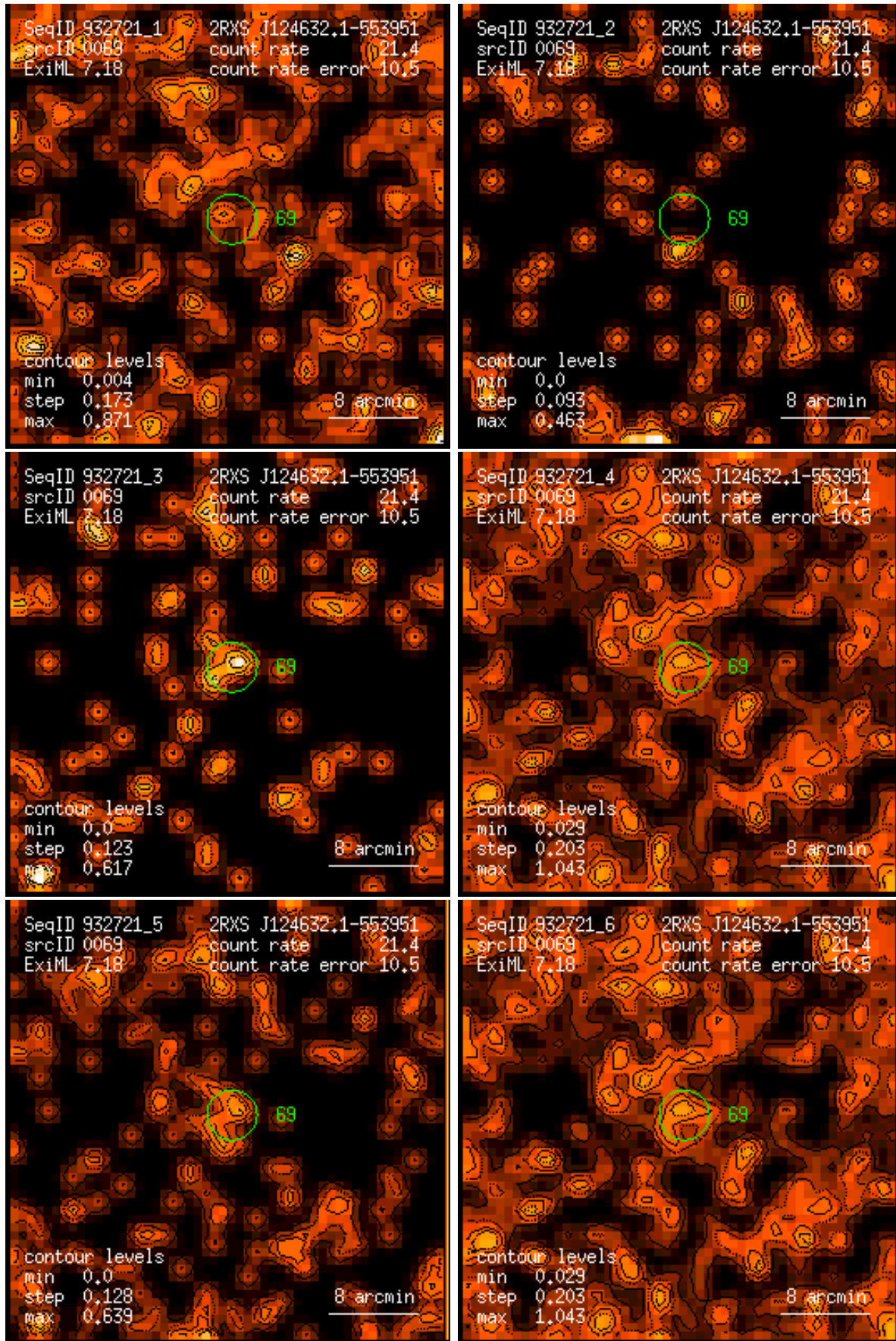
Figure 69: RASS 932721: detection 0069: band rate images, Gaussian filter: (1) PSPC channels 11 – 41, (2) 52 – 90, (3) 91 – 201, (4) 11 – 235, (5) 52 – 201, (6) 11 – 201. Broad band rates in counts/ks. Band rate contour levels in counts/ks/arcmin 2 .
