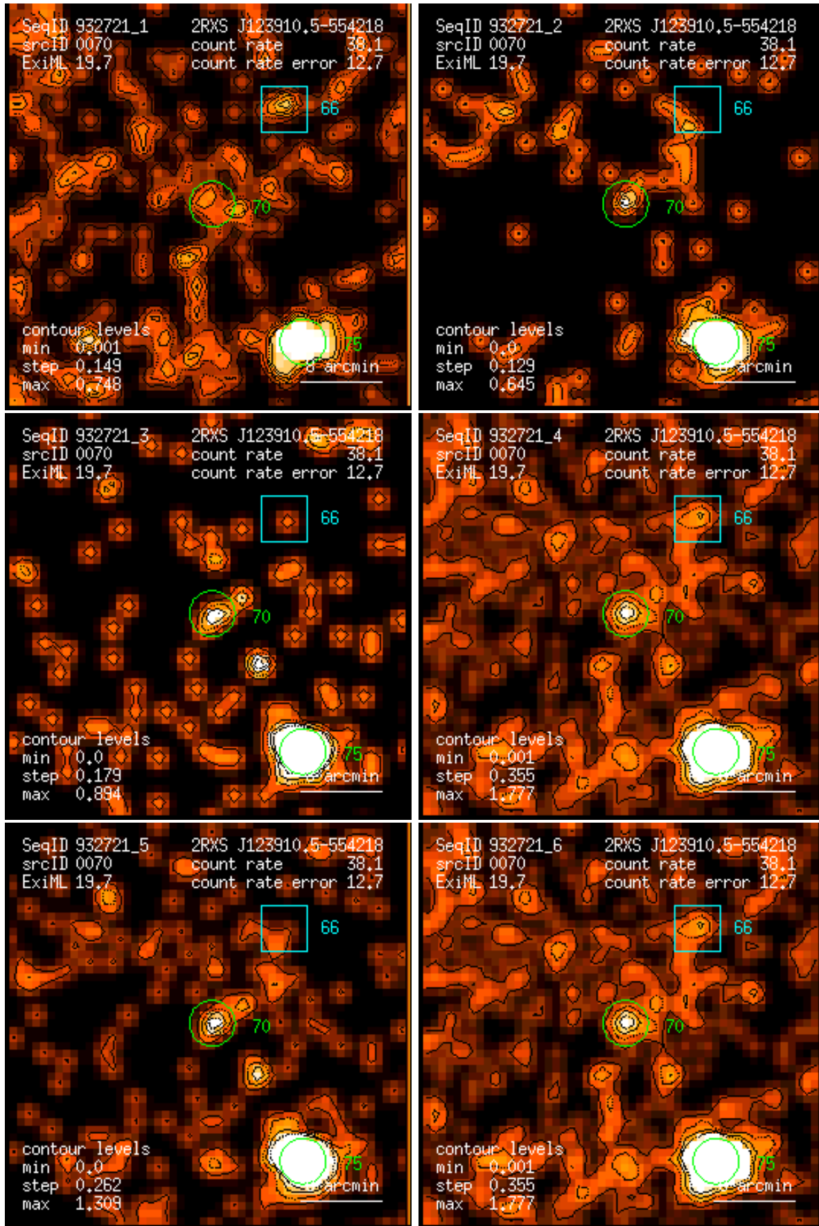
Figure 70: RASS 932721: detection 0070: band rate images, Gaussian filter: (1) PSPC channels 11 – 41, (2) 52 – 90, (3) 91 – 201, (4) 11 – 235, (5) 52 – 201, (6) 11 – 201. Broad band rates in counts/ks. Band rate contour levels in counts/ks/arcmin 2 .
