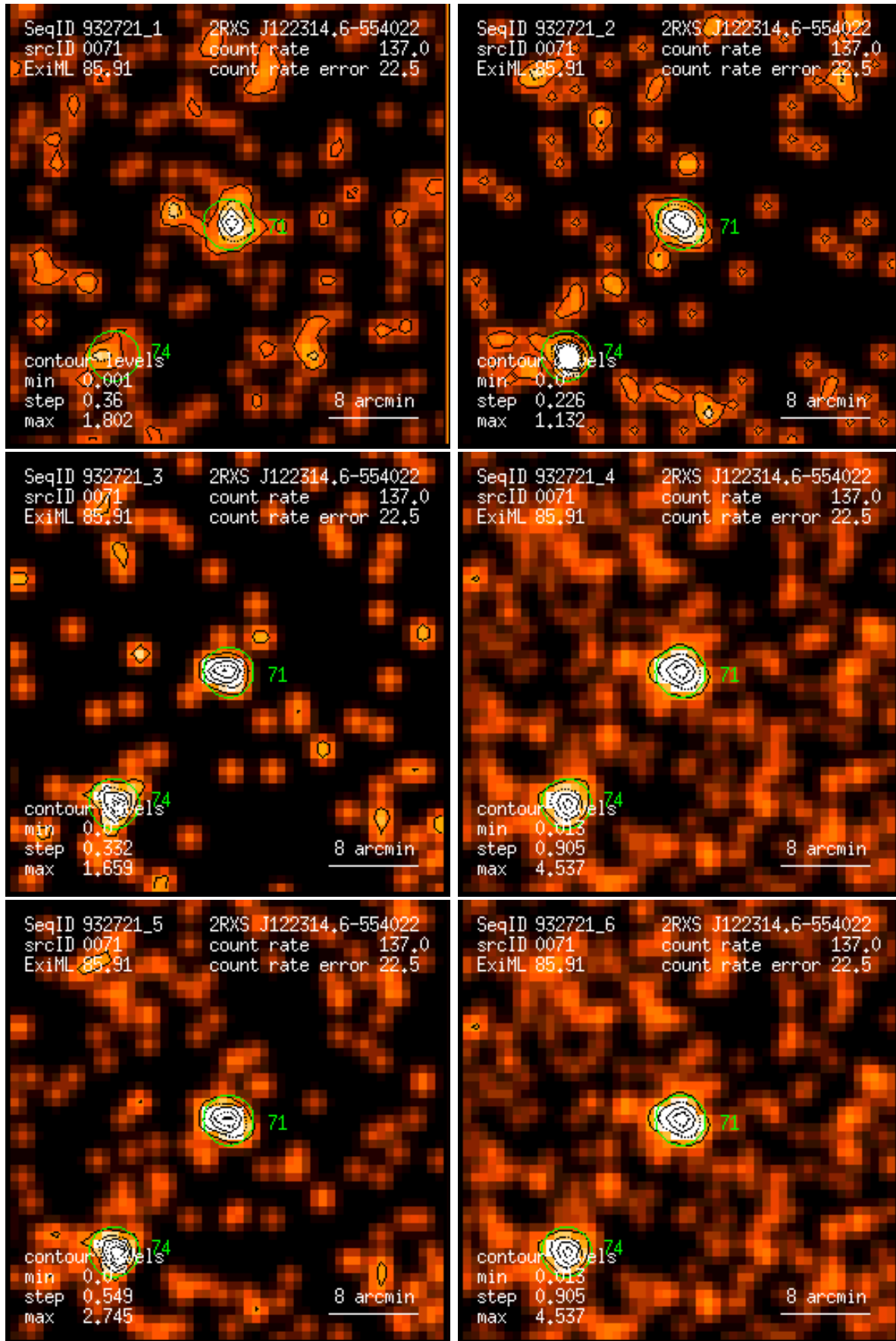
Figure 71: RASS 932721: detection 0071: band rate images, Gaussian filter: (1) PSPC channels 11 – 41, (2) 52 – 90, (3) 91 – 201, (4) 11 – 235, (5) 52 – 201, (6) 11 – 201. Broad band rates in counts/ks. Band rate contour levels in counts/ks/arcmin 2 .
