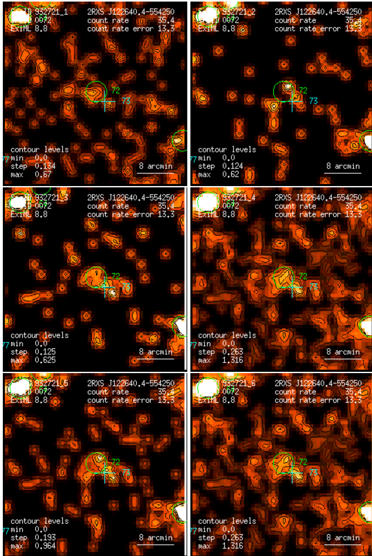
Figure 72: RASS 932721: detection 0072: band rate images, Gaussian filter: (1) PSPC channels 11 – 41, (2) 52 – 90, (3) 91 – 201, (4) 11 – 235, (5) 52 – 201, (6) 11 – 201. Broad band rates in counts/ks. Band rate contour levels in counts/ks/arcmin 2 .
