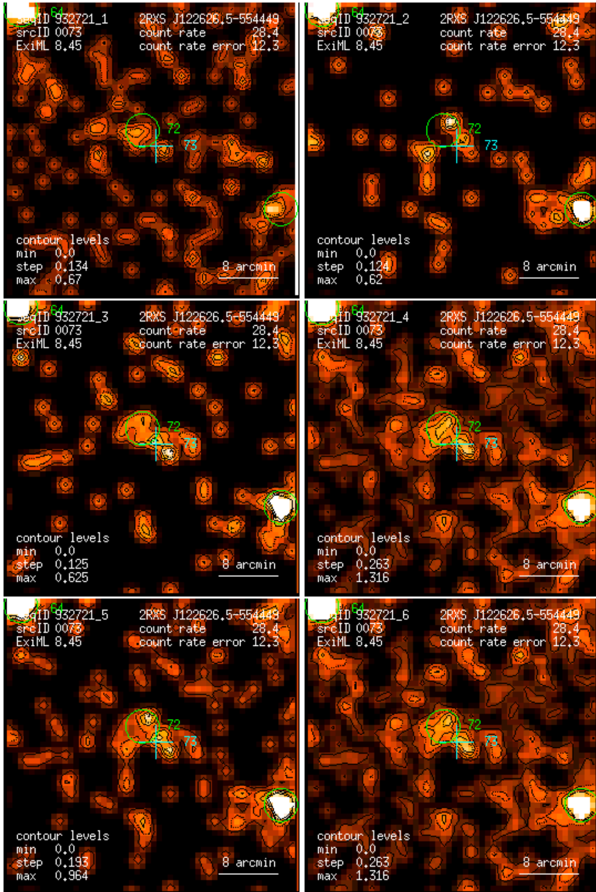
Figure 73: RASS 932721: detection 0073: band rate images, Gaussian filter: (1) PSPC channels 11 – 41, (2) 52 – 90, (3) 91 – 201, (4) 11 – 235, (5) 52 – 201, (6) 11 – 201. Broad band rates in counts/ks. Band rate contour levels in counts/ks/arcmin 2 .
