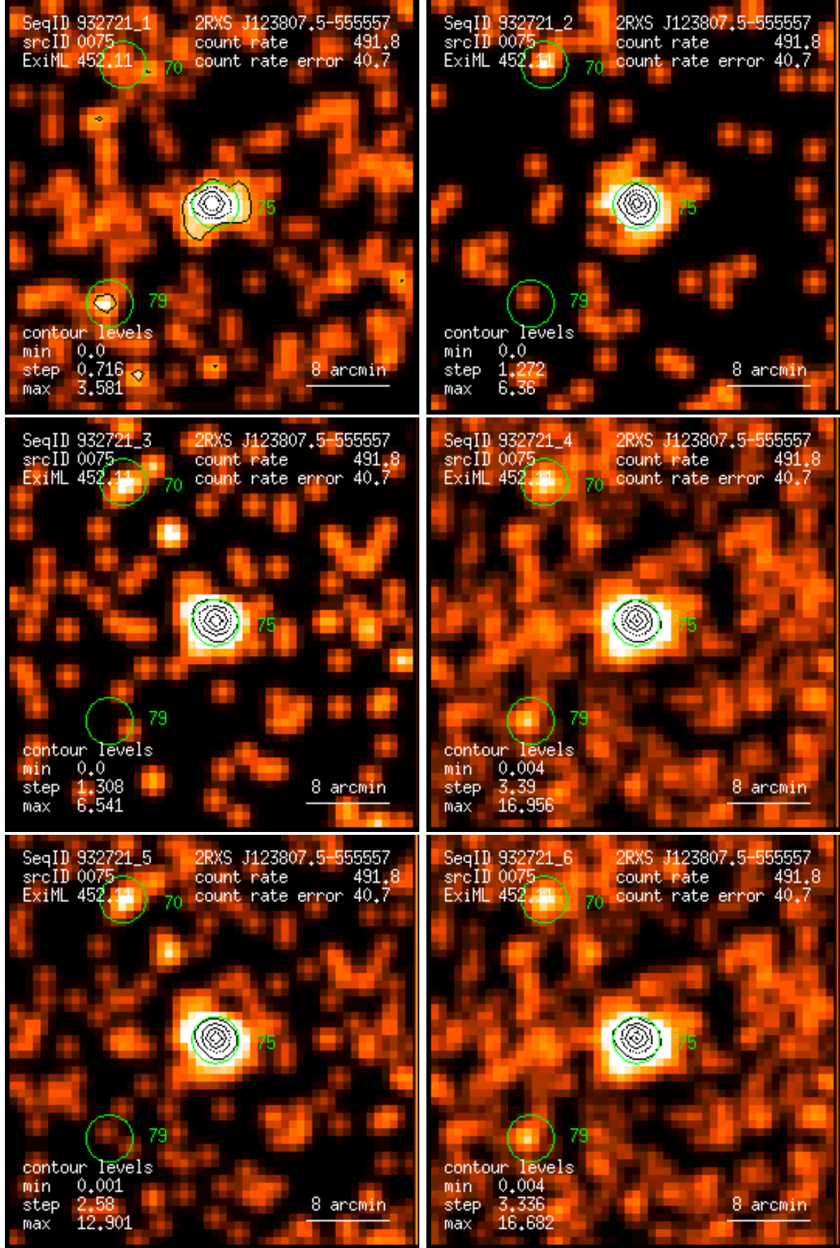
Figure 75: RASS 932721: detection 0075: band rate images, Gaussian filter: (1) PSPC channels 11 – 41, (2) 52 – 90, (3) 91 – 201, (4) 11 – 235, (5) 52 – 201, (6) 11 – 201. Broad band rates in counts/ks. Band rate contour levels in counts/ks/arcmin 2 .
