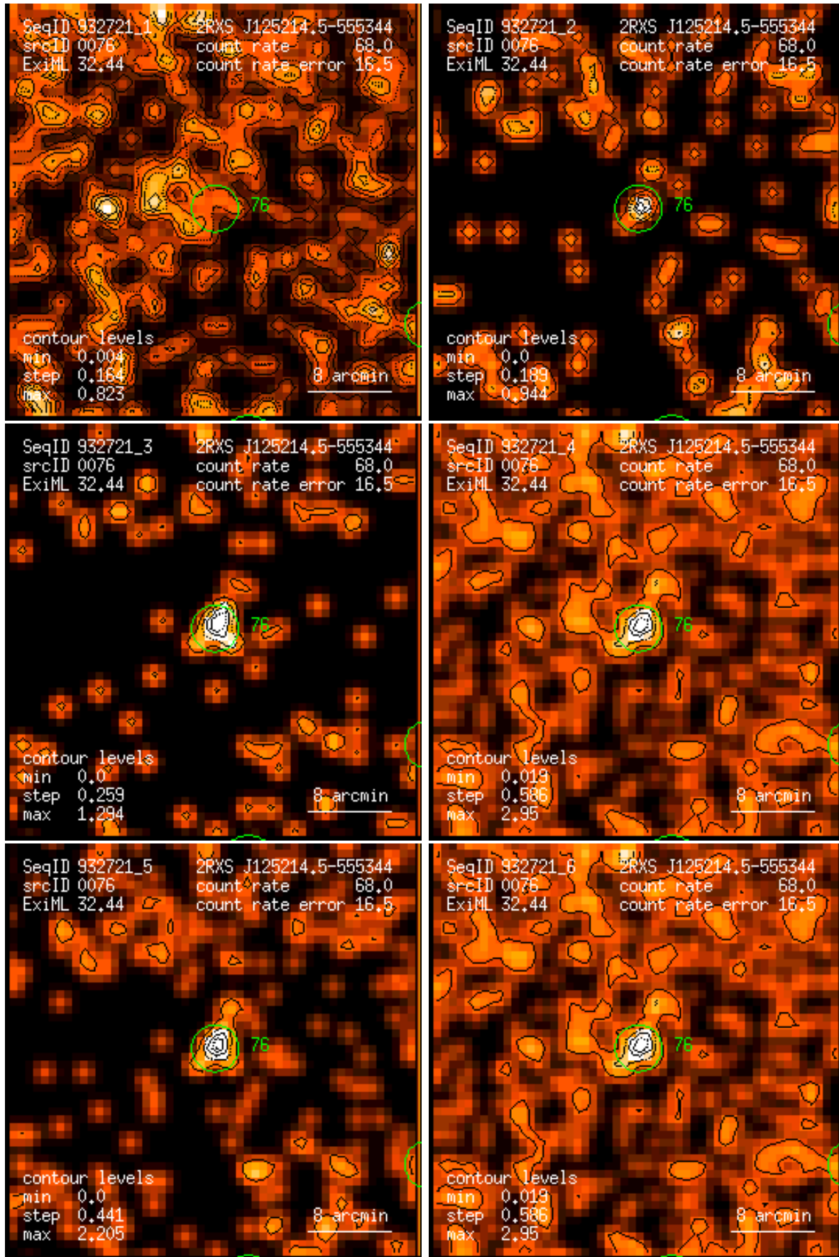
Figure 76: RASS 932721: detection 0076: band rate images, Gaussian filter: (1) PSPC channels 11 – 41, (2) 52 – 90, (3) 91 – 201, (4) 11 – 235, (5) 52 – 201, (6) 11 – 201. Broad band rates in counts/ks. Band rate contour levels in counts/ks/arcmin 2 .
