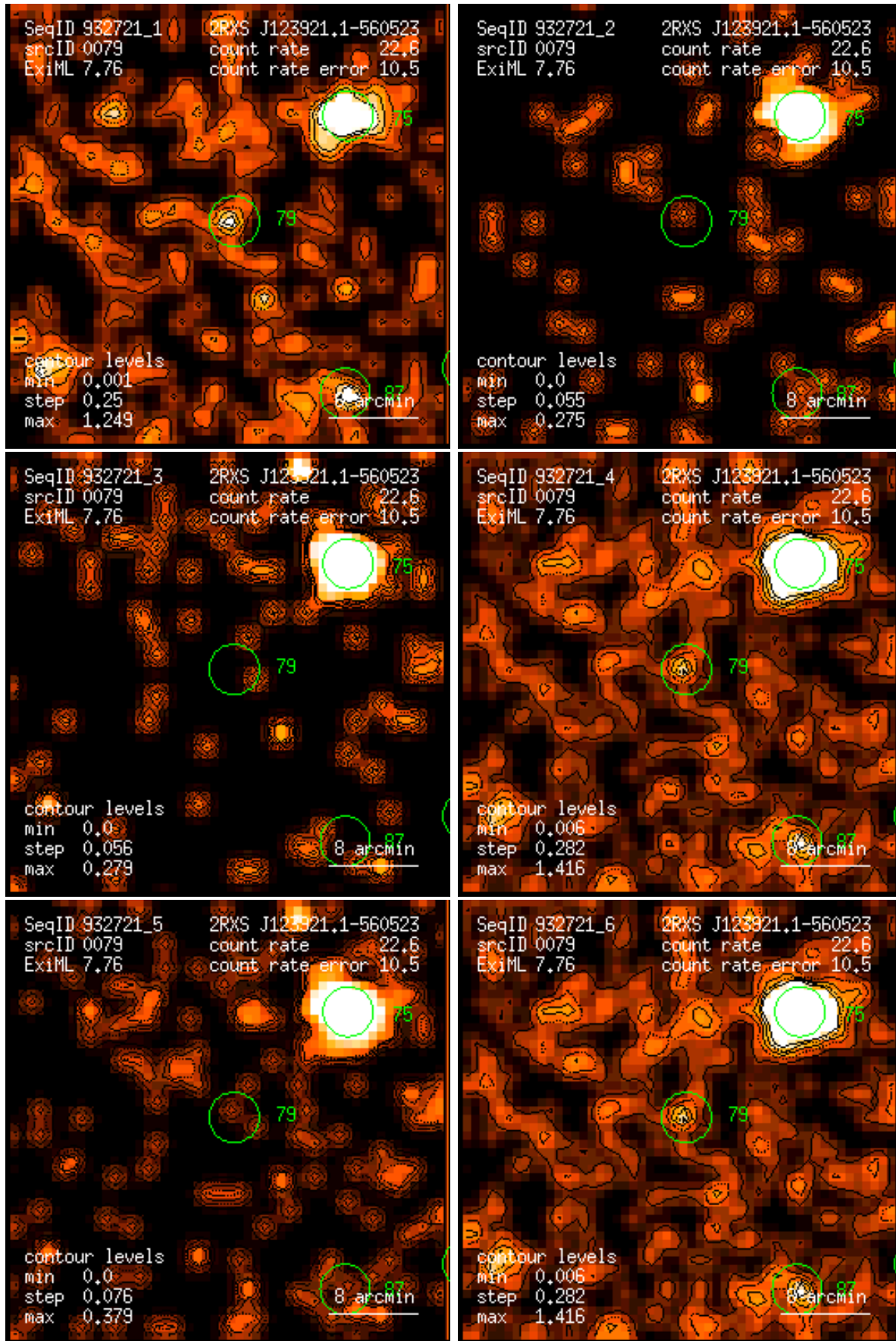
Figure 79: RASS 932721: detection 0079: band rate images, Gaussian filter: (1) PSPC channels 11 – 41, (2) 52 – 90, (3) 91 – 201, (4) 11 – 235, (5) 52 – 201, (6) 11 – 201. Broad band rates in counts/ks. Band rate contour levels in counts/ks/arcmin 2 .
