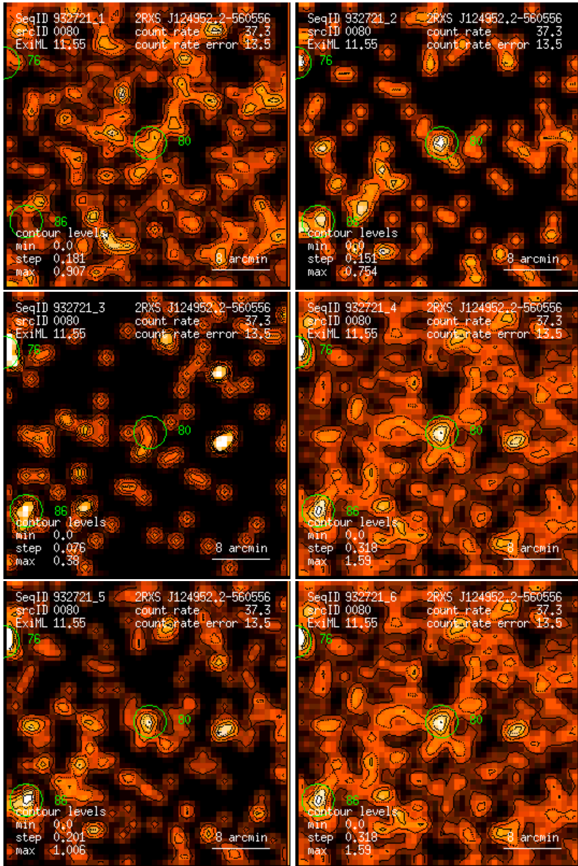
Figure 80: RASS 932721: detection 0080: band rate images, Gaussian filter: (1) PSPC channels 11 – 41, (2) 52 – 90, (3) 91 – 201, (4) 11 – 235, (5) 52 – 201, (6) 11 – 201. Broad band rates in counts/ks. Band rate contour levels in counts/ks/arcmin 2 .
