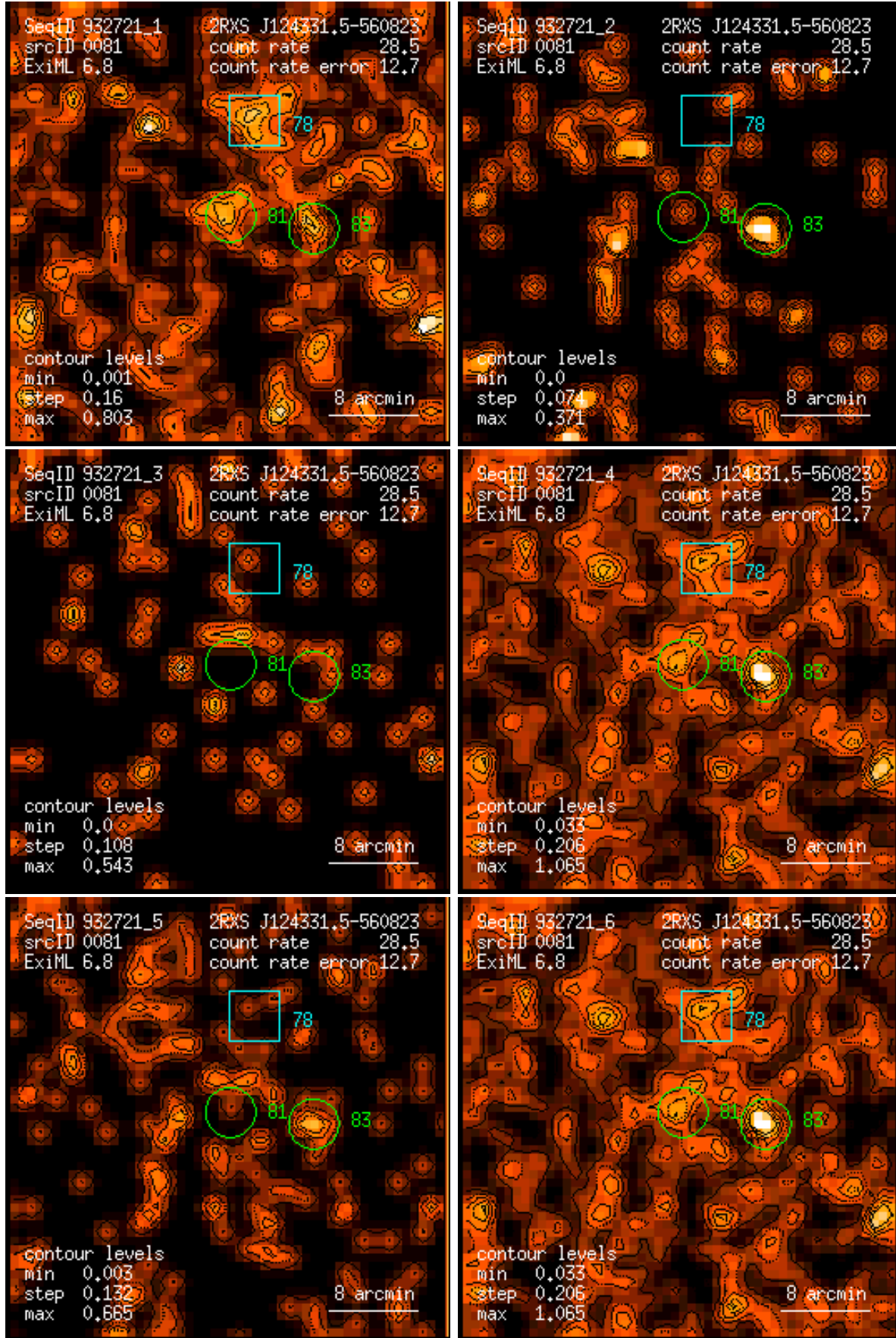
Figure 81: RASS 932721: detection 0081: band rate images, Gaussian filter: (1) PSPC channels 11 – 41, (2) 52 – 90, (3) 91 – 201, (4) 11 – 235, (5) 52 – 201, (6) 11 – 201. Broad band rates in counts/ks. Band rate contour levels in counts/ks/arcmin 2 .
