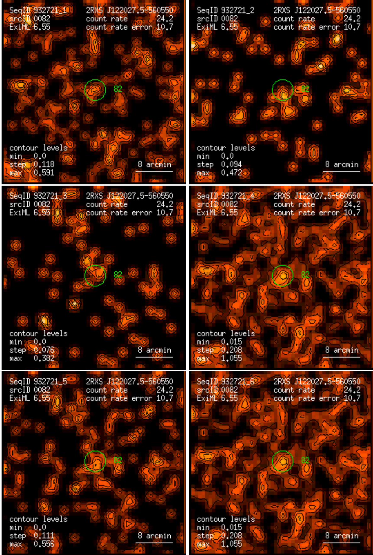
Figure 82: RASS 932721: detection 0082: band rate images, Gaussian filter: (1) PSPC channels 11 – 41, (2) 52 – 90, (3) 91 – 201, (4) 11 – 235, (5) 52 – 201, (6) 11 – 201. Broad band rates in counts/ks. Band rate contour levels in counts/ks/arcmin 2 .
