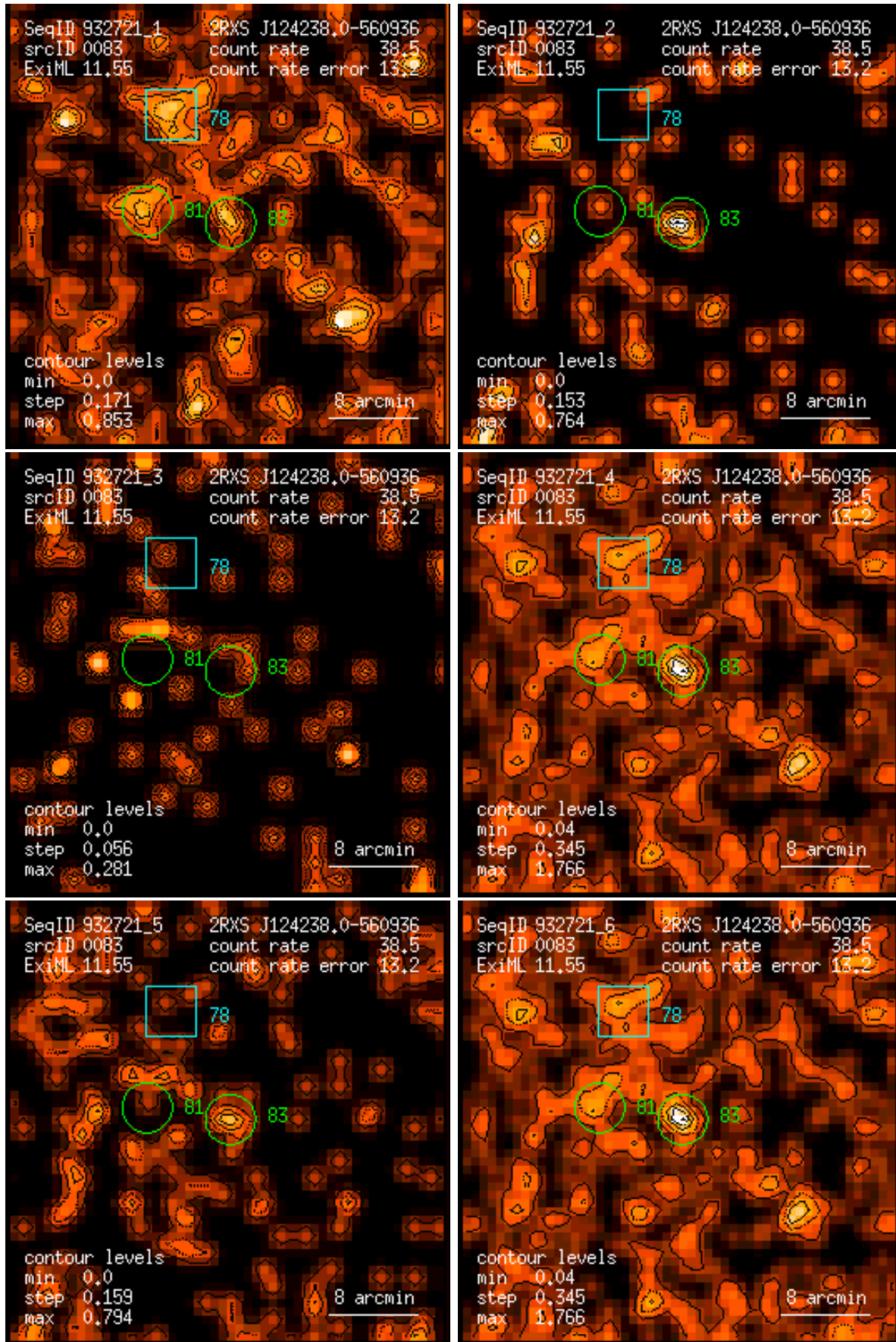
Figure 83: RASS 932721: detection 0083: band rate images, Gaussian filter: (1) PSPC channels 11 – 41, (2) 52 – 90, (3) 91 – 201, (4) 11 – 235, (5) 52 – 201, (6) 11 – 201. Broad band rates in counts/ks. Band rate contour levels in counts/ks/arcmin 2 .
