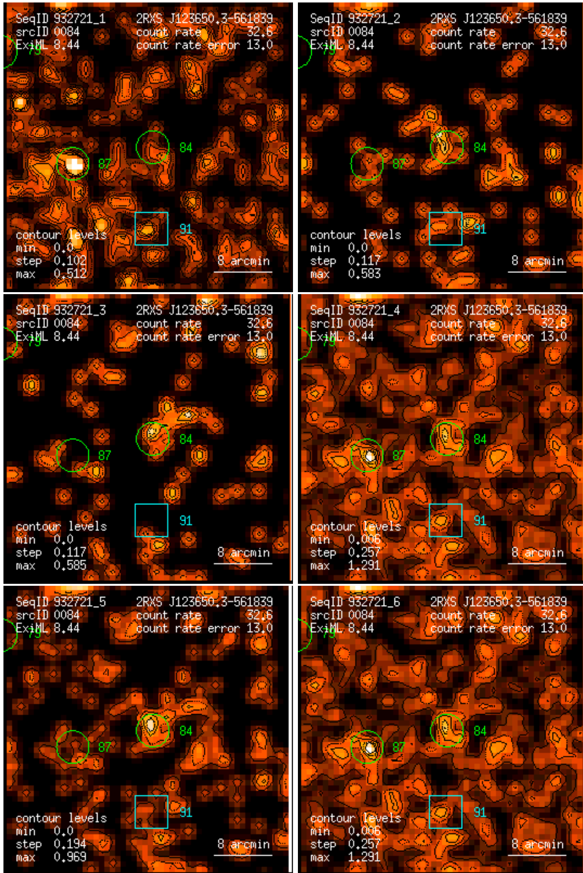
Figure 84: RASS 932721: detection 0084: band rate images, Gaussian filter: (1) PSPC channels 11 – 41, (2) 52 – 90, (3) 91 – 201, (4) 11 – 235, (5) 52 – 201, (6) 11 – 201. Broad band rates in counts/ks. Band rate contour levels in counts/ks/arcmin 2 .
