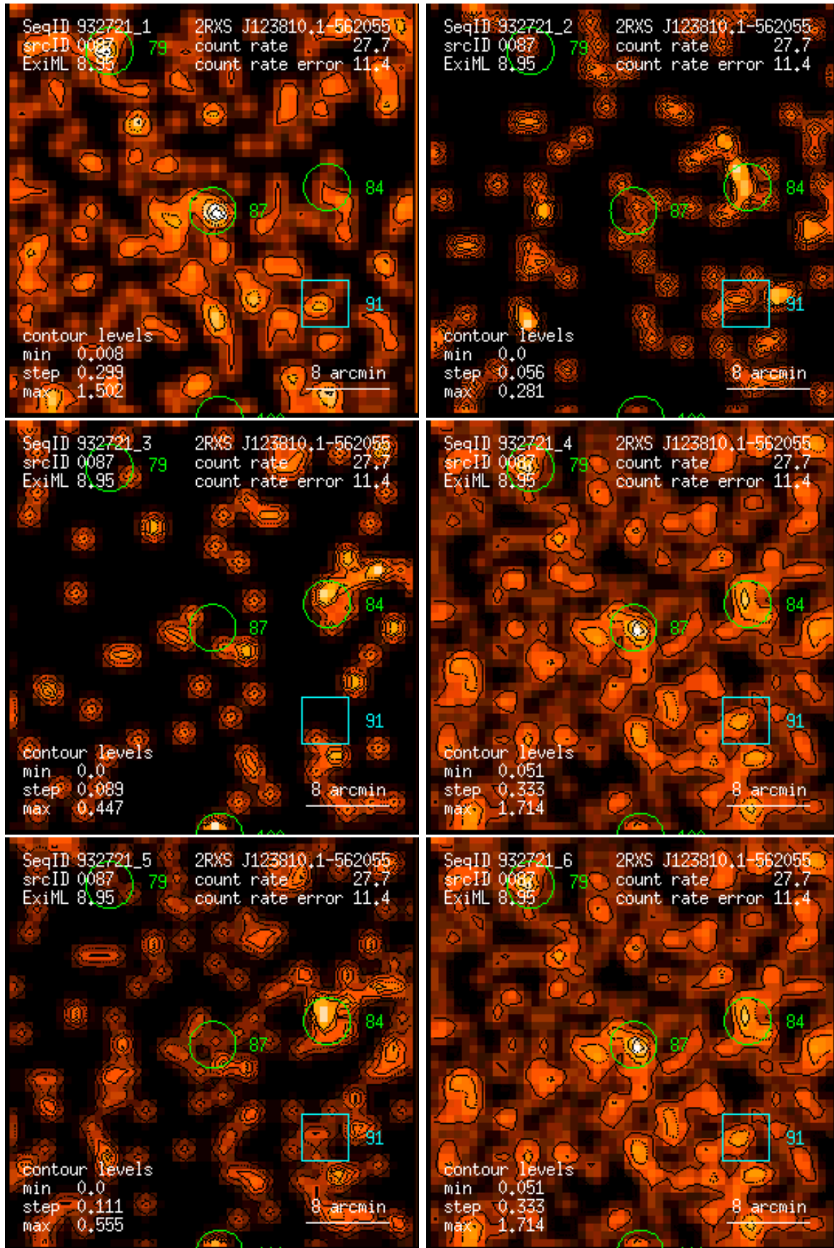
Figure 87: RASS 932721: detection 0087: band rate images, Gaussian filter: (1) PSPC channels 11 – 41, (2) 52 – 90, (3) 91 – 201, (4) 11 – 235, (5) 52 – 201, (6) 11 – 201. Broad band rates in counts/ks. Band rate contour levels in counts/ks/arcmin 2 .
