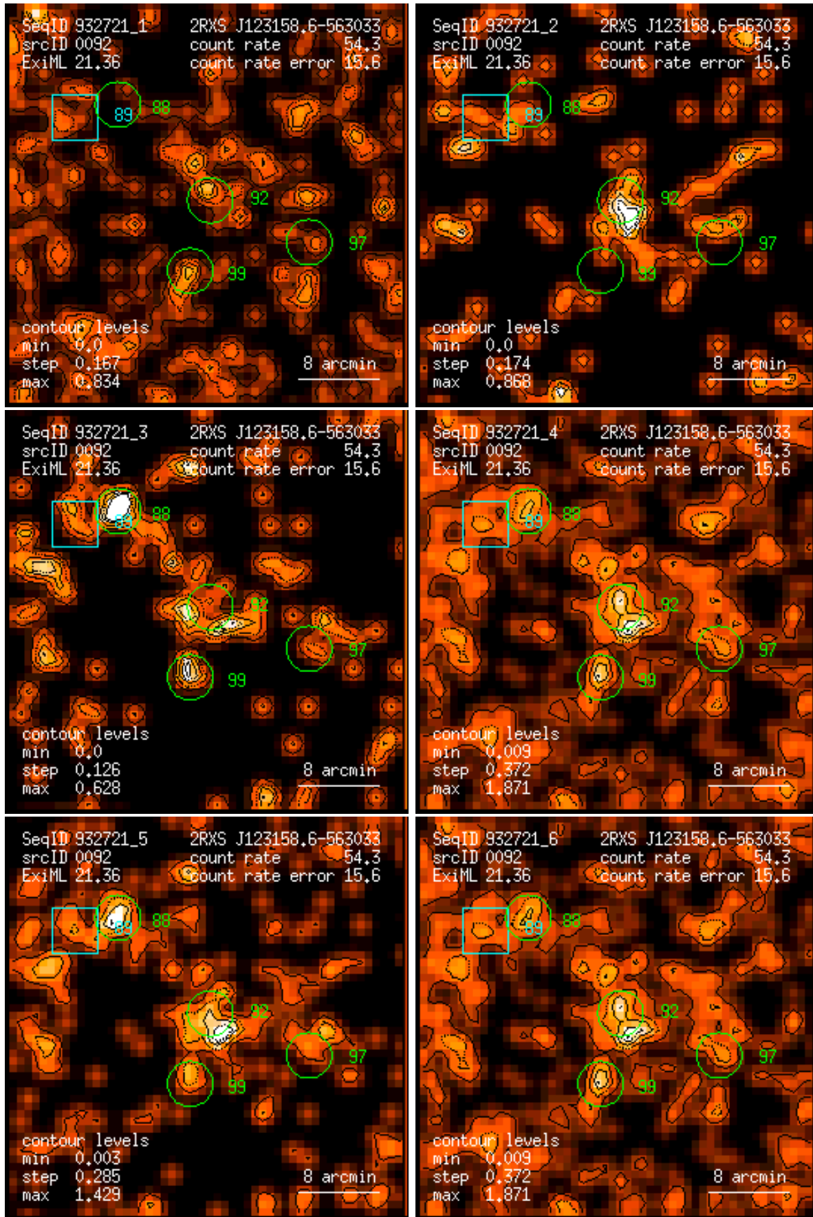
Figure 92: RASS 932721: detection 0092: band rate images, Gaussian filter: (1) PSPC channels 11 – 41, (2) 52 – 90, (3) 91 – 201, (4) 11 – 235, (5) 52 – 201, (6) 11 – 201. Broad band rates in counts/ks. Band rate contour levels in counts/ks/arcmin 2 .
