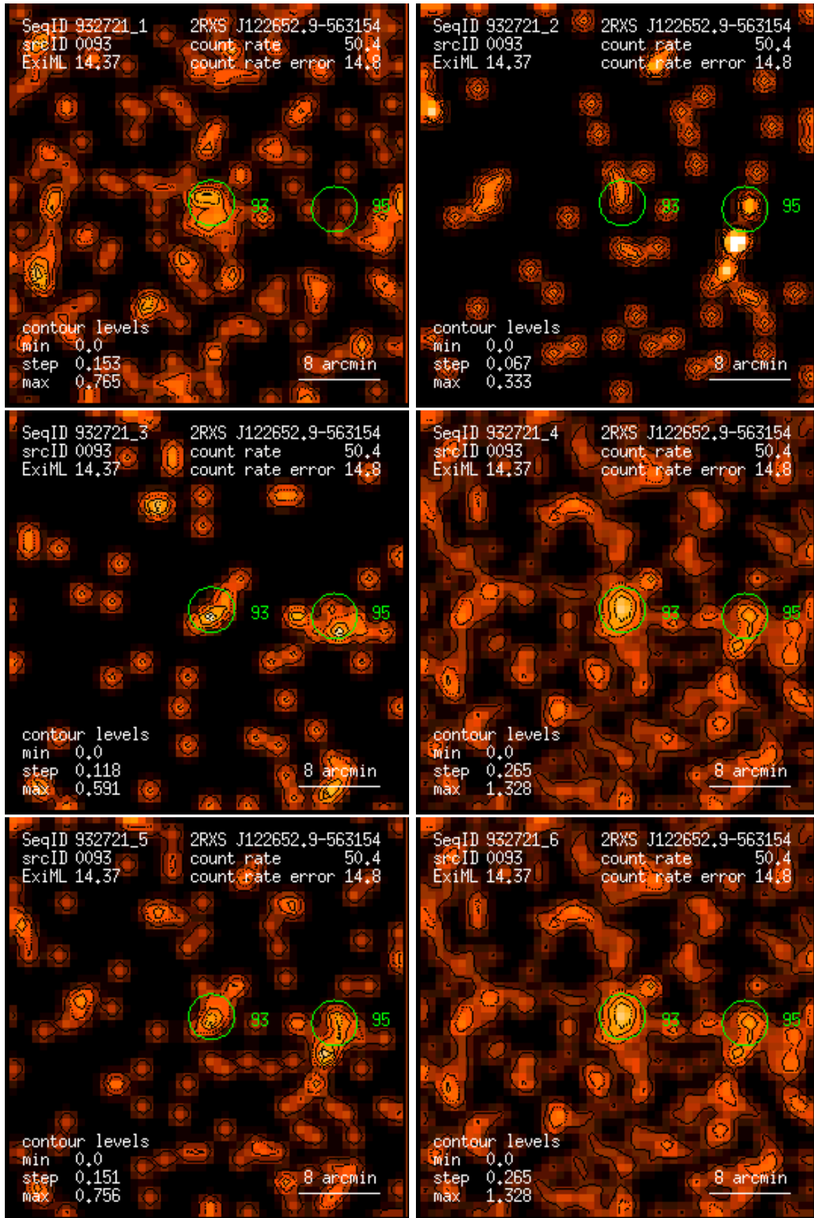
Figure 93: RASS 932721: detection 0093: band rate images, Gaussian filter: (1) PSPC channels 11 – 41, (2) 52 – 90, (3) 91 – 201, (4) 11 – 235, (5) 52 – 201, (6) 11 – 201. Broad band rates in counts/ks. Band rate contour levels in counts/ks/arcmin 2 .
