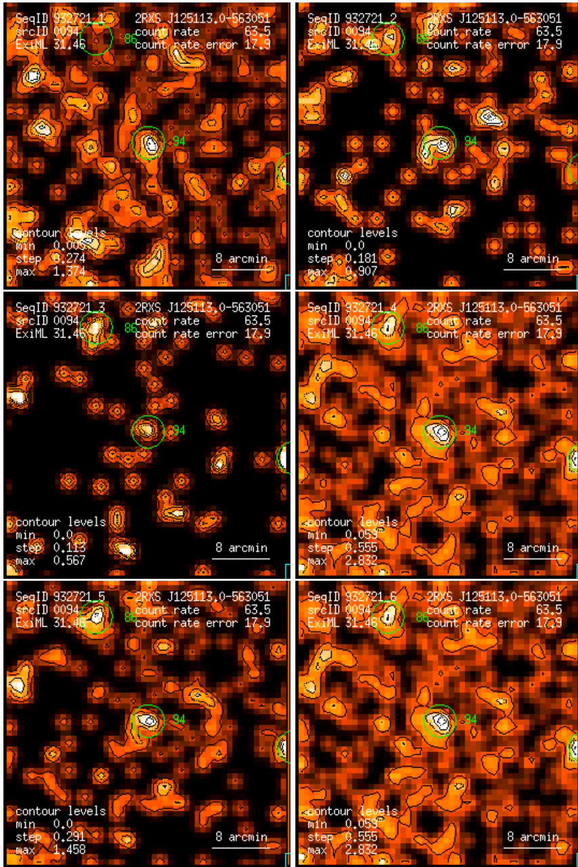
Figure 94: RASS 932721: detection 0094: band rate images, Gaussian filter: (1) PSPC channels 11 – 41, (2) 52 – 90, (3) 91 – 201, (4) 11 – 235, (5) 52 – 201, (6) 11 – 201. Broad band rates in counts/ks. Band rate contour levels in counts/ks/arcmin 2 .
