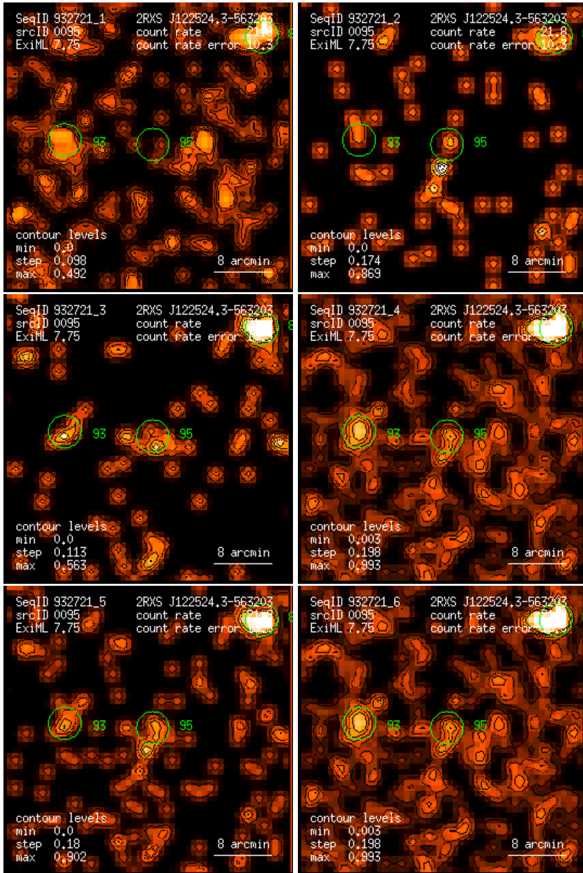
Figure 95: RASS 932721: detection 0095: band rate images, Gaussian filter: (1) PSPC channels 11 – 41, (2) 52 – 90, (3) 91 – 201, (4) 11 – 235, (5) 52 – 201, (6) 11 – 201. Broad band rates in counts/ks. Band rate contour levels in counts/ks/arcmin 2 .
