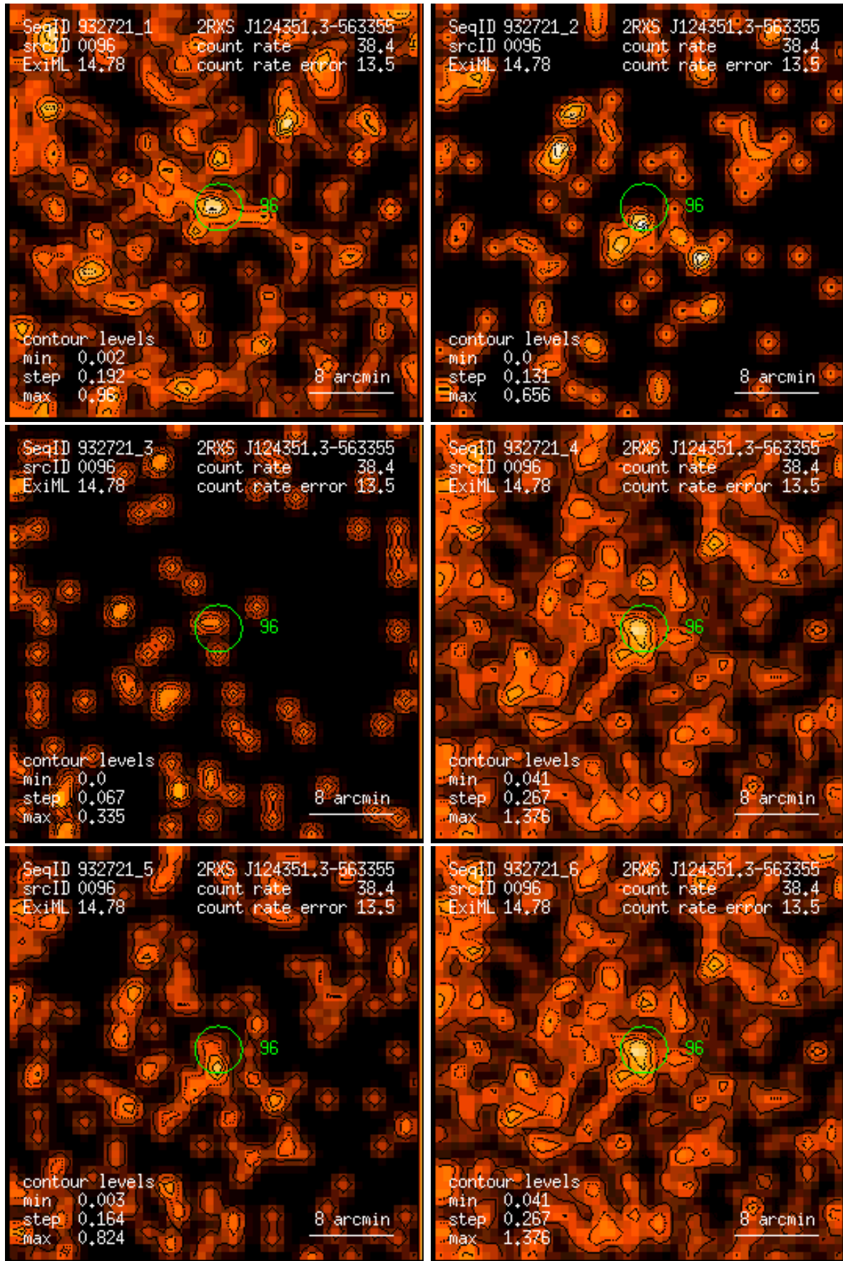
Figure 96: RASS 932721: detection 0096: band rate images, Gaussian filter: (1) PSPC channels 11 – 41, (2) 52 – 90, (3) 91 – 201, (4) 11 – 235, (5) 52 – 201, (6) 11 – 201. Broad band rates in counts/ks. Band rate contour levels in counts/ks/arcmin 2 .
