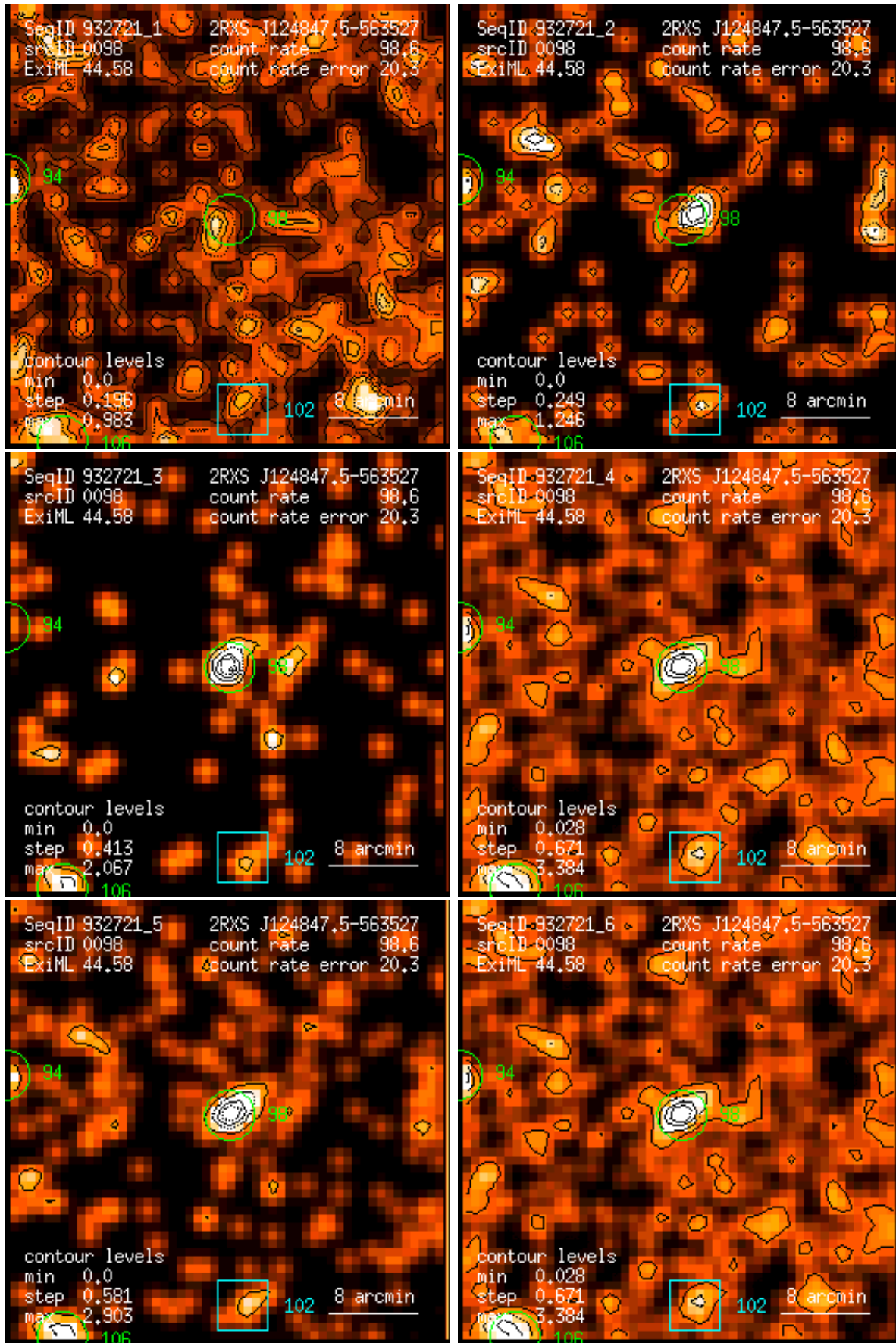
Figure 98: RASS 932721: detection 0098: band rate images, Gaussian filter: (1) PSPC channels 11 – 41, (2) 52 – 90, (3) 91 – 201, (4) 11 – 235, (5) 52 – 201, (6) 11 – 201. Broad band rates in counts/ks. Band rate contour levels in counts/ks/arcmin 2 .
