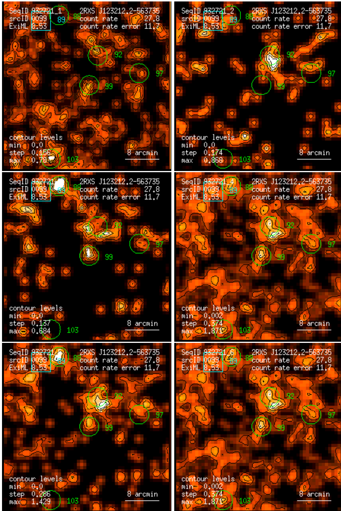
Figure 99: RASS 932721: detection 0099: band rate images, Gaussian filter: (1) PSPC channels 11 – 41, (2) 52 – 90, (3) 91 – 201, (4) 11 – 235, (5) 52 – 201, (6) 11 – 201. Broad band rates in counts/ks. Band rate contour levels in counts/ks/arcmin 2 .
