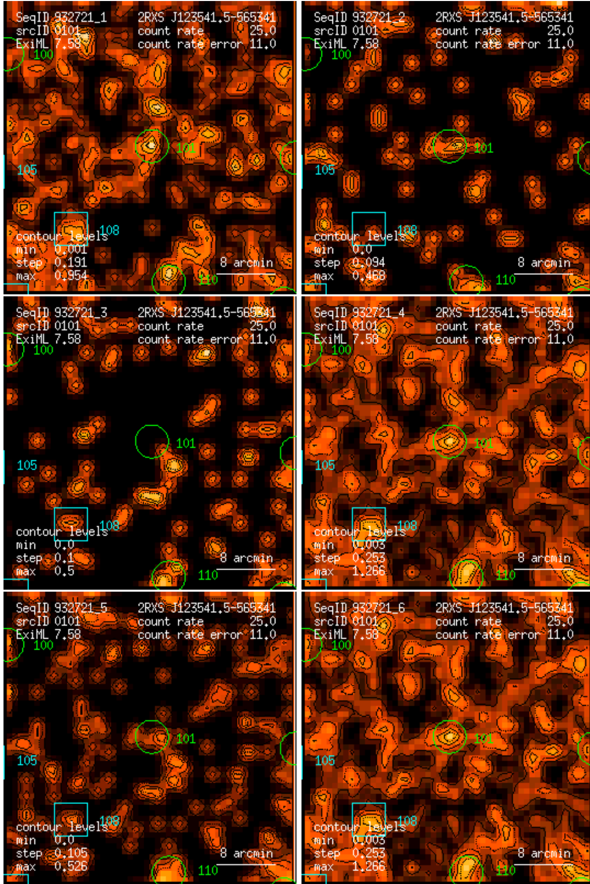
Figure 101: RASS 932721: detection 0101: band rate images, Gaussian filter: (1) PSPC channels 11 – 41, (2) 52 – 90, (3) 91 – 201, (4) 11 – 235, (5) 52 – 201, (6) 11 – 201. Broad band rates in counts/ks. Band rate contour levels in counts/ks/arcmin 2 .
