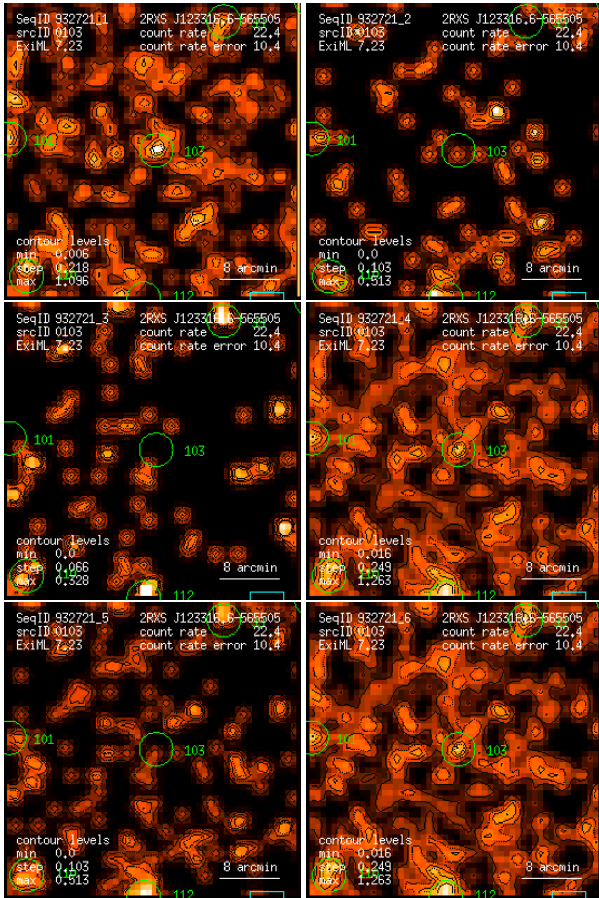
Figure 103: RASS 932721: detection 0103: band rate images, Gaussian filter: (1) PSPC channels 11 – 41, (2) 52 – 90, (3) 91 – 201, (4) 11 – 235, (5) 52 – 201, (6) 11 – 201. Broad band rates in counts/ks. Band rate contour levels in counts/ks/arcmin 2 .
