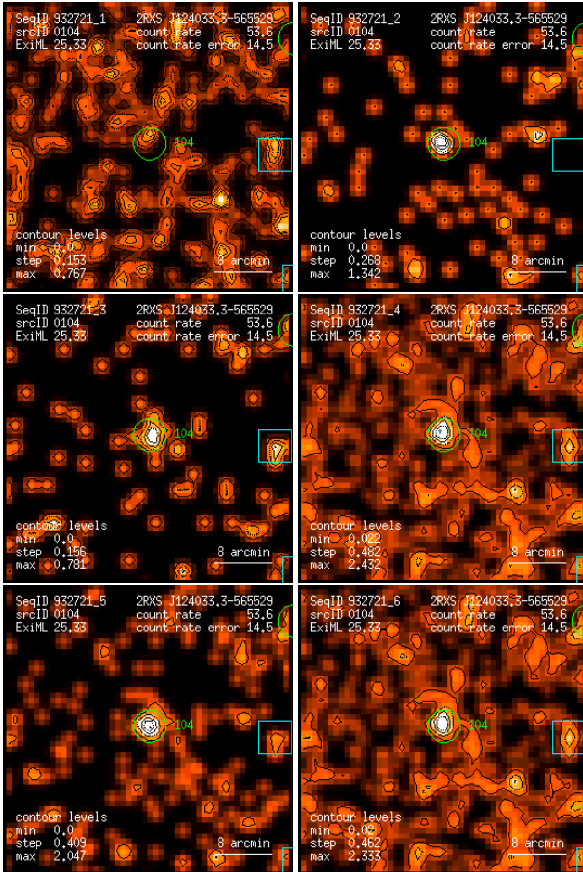
Figure 104: RASS 932721: detection 0104: band rate images, Gaussian filter: (1) PSPC channels 11 – 41, (2) 52 – 90, (3) 91 – 201, (4) 11 – 235, (5) 52 – 201, (6) 11 – 201. Broad band rates in counts/ks. Band rate contour levels in counts/ks/arcmin 2 .
