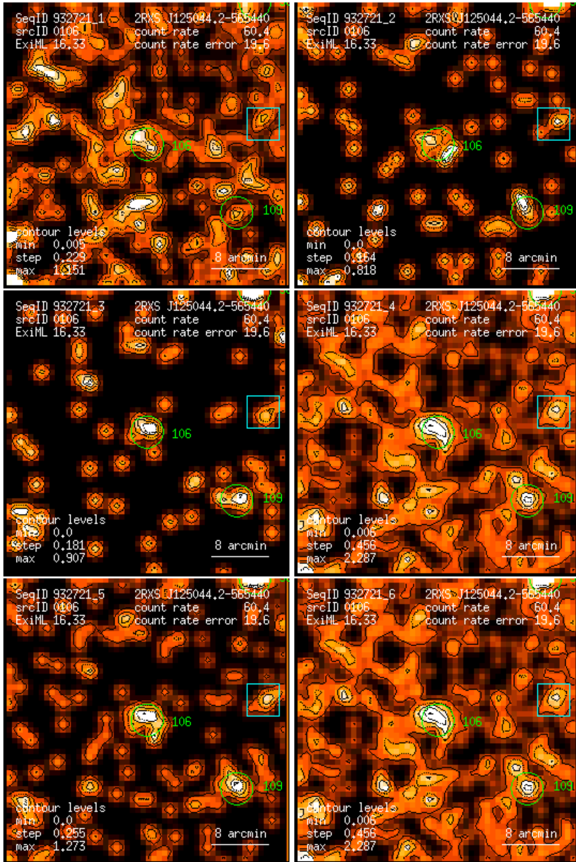
Figure 106: RASS 932721: detection 0106: band rate images, Gaussian filter: (1) PSPC channels 11 – 41, (2) 52 – 90, (3) 91 – 201, (4) 11 – 235, (5) 52 – 201, (6) 11 – 201. Broad band rates in counts/ks. Band rate contour levels in counts/ks/arcmin 2 .
