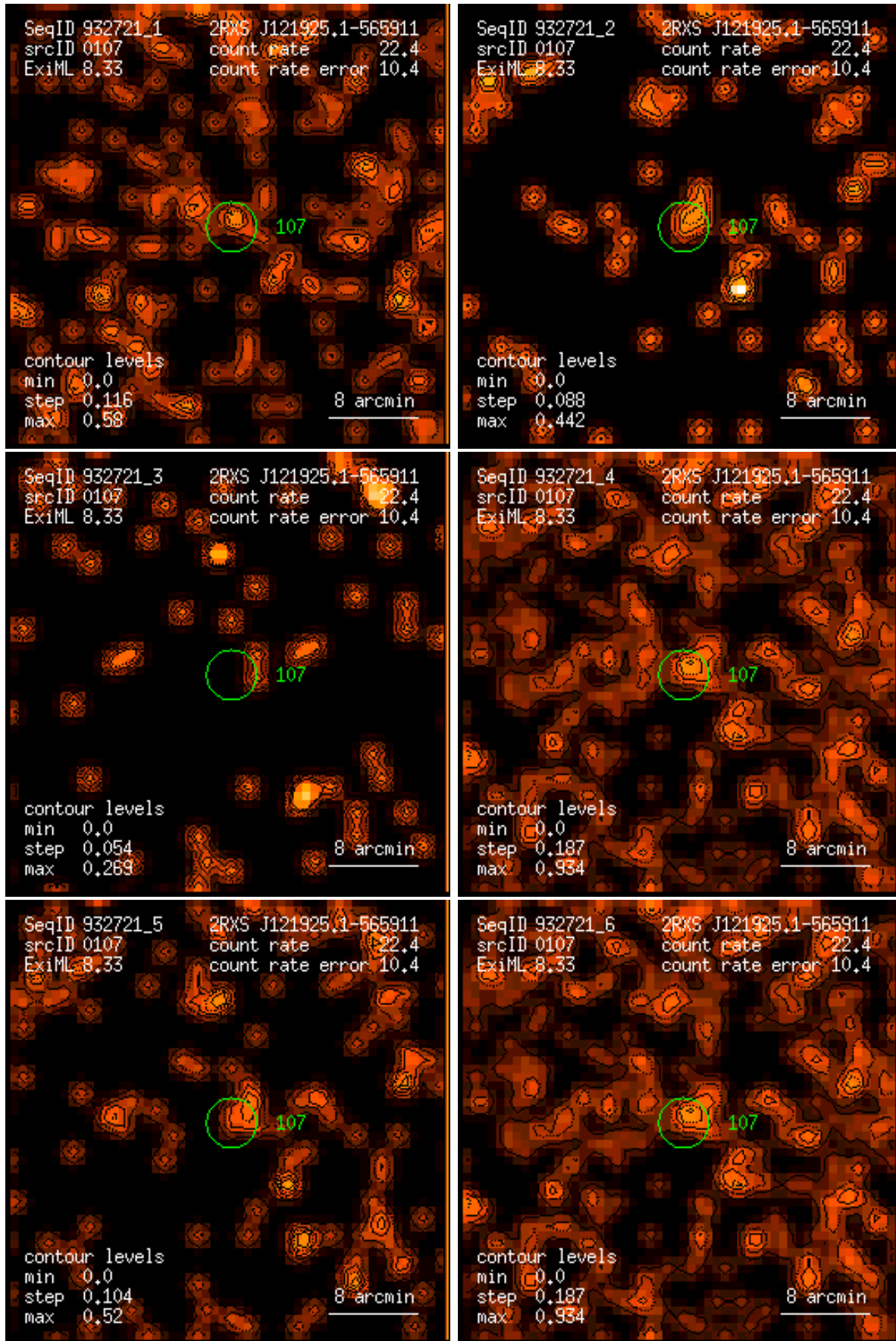
Figure 107: RASS 932721: detection 0107: band rate images, Gaussian filter: (1) PSPC channels 11 – 41, (2) 52 – 90, (3) 91 – 201, (4) 11 – 235, (5) 52 – 201, (6) 11 – 201. Broad band rates in counts/ks. Band rate contour levels in counts/ks/arcmin 2 .
