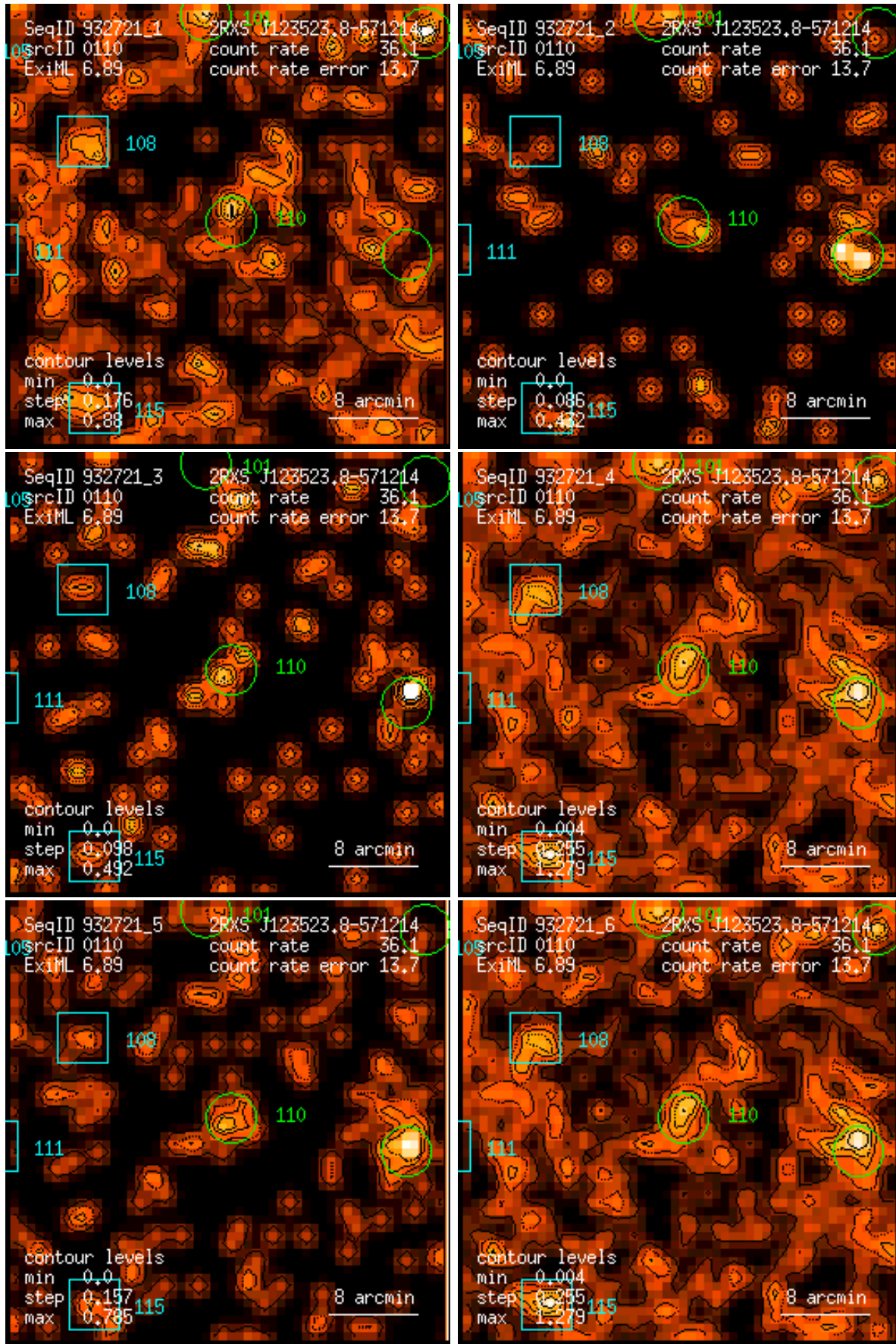
Figure 110: RASS 932721: detection 0110: band rate images, Gaussian filter: (1) PSPC channels 11 – 41, (2) 52 – 90, (3) 91 – 201, (4) 11 – 235, (5) 52 – 201, (6) 11 – 201. Broad band rates in counts/ks. Band rate contour levels in counts/ks/arcmin 2 .
