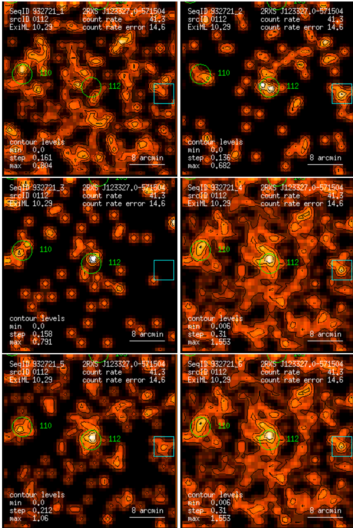
Figure 112: RASS 932721: detection 0112: band rate images, Gaussian filter: (1) PSPC channels 11 – 41, (2) 52 – 90, (3) 91 – 201, (4) 11 – 235, (5) 52 – 201, (6) 11 – 201. Broad band rates in counts/ks. Band rate contour levels in counts/ks/arcmin 2 .
