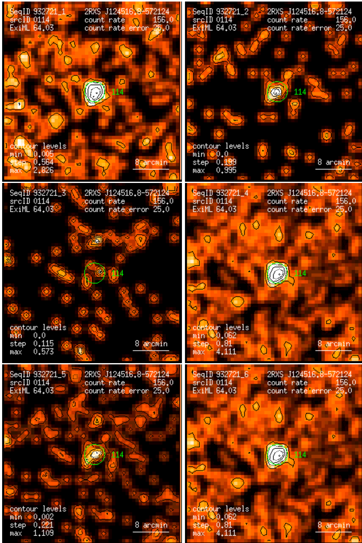
Figure 114: RASS 932721: detection 0114: band rate images, Gaussian filter: (1) PSPC channels 11 – 41, (2) 52 – 90, (3) 91 – 201, (4) 11 – 235, (5) 52 – 201, (6) 11 – 201. Broad band rates in counts/ks. Band rate contour levels in counts/ks/arcmin 2 .
