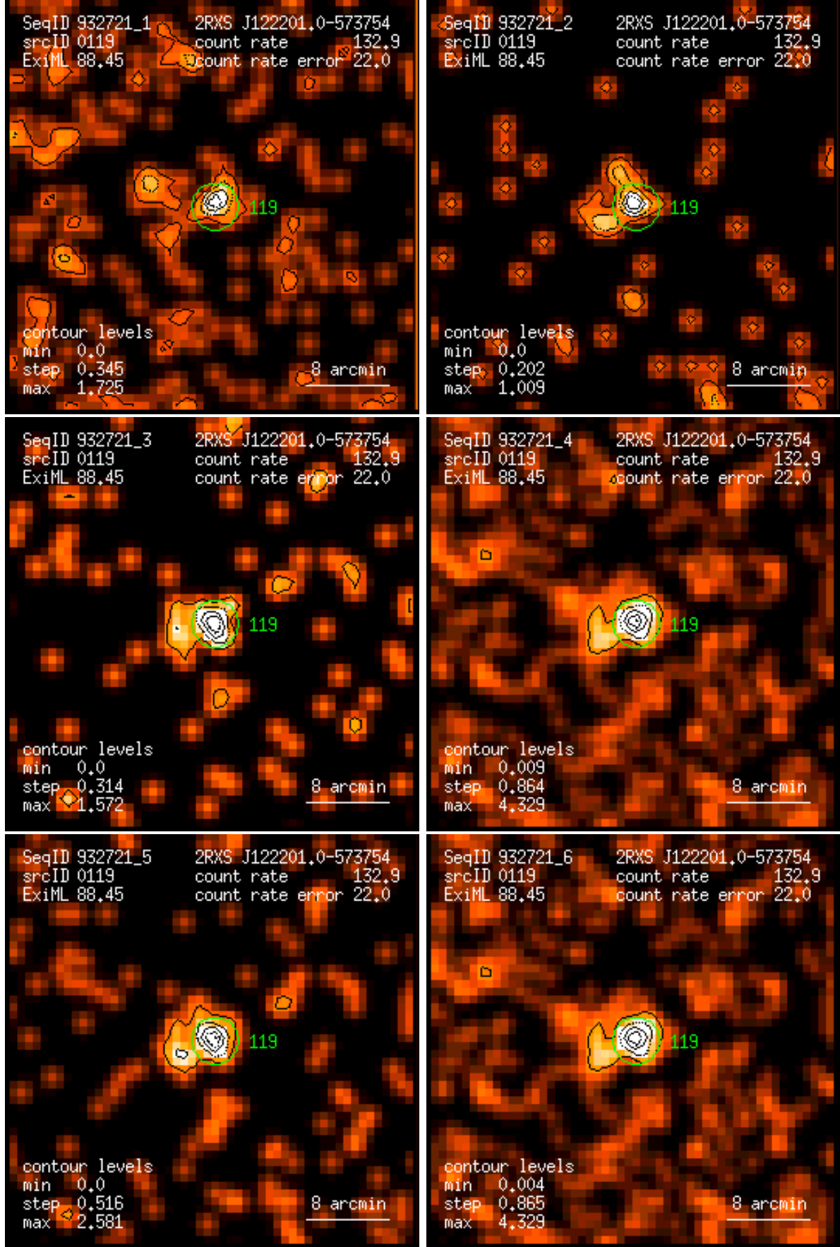
Figure 119: RASS 932721: detection 0119: band rate images, Gaussian filter: (1) PSPC channels 11 – 41, (2) 52 – 90, (3) 91 – 201, (4) 11 – 235, (5) 52 – 201, (6) 11 – 201. Broad band rates in counts/ks. Band rate contour levels in counts/ks/arcmin 2 .
